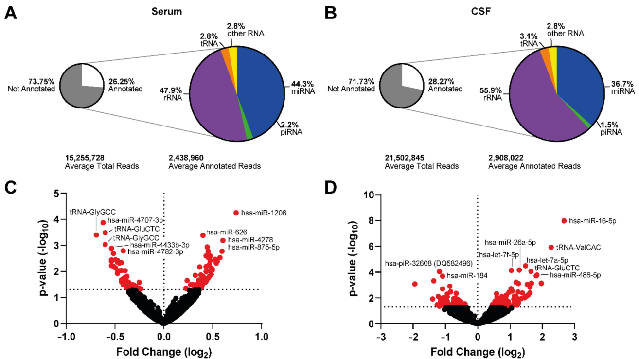
Figure 1. RNA-seq shows ncRNA may be dysregulated in the serum and CSF from PSP patients compared to healthy controls. Summary of the number of aligned reads that were annotated and the ncRNA species they aligned to in serum (A) and CSF (B) with volcano plots of ncRNA dysregulated in serum (C) and CSF (D). Dots in red were significantly dysregulated compared to healthy control, with the ten most significantly dysregulated labelled.
