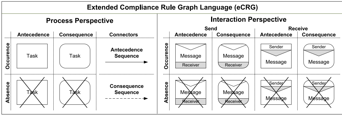
Fig. 6. Elements of the eCRG language.
