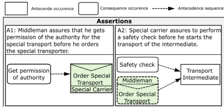
Fig. 5. Assertions by partners Middleman and Special Carrier .
