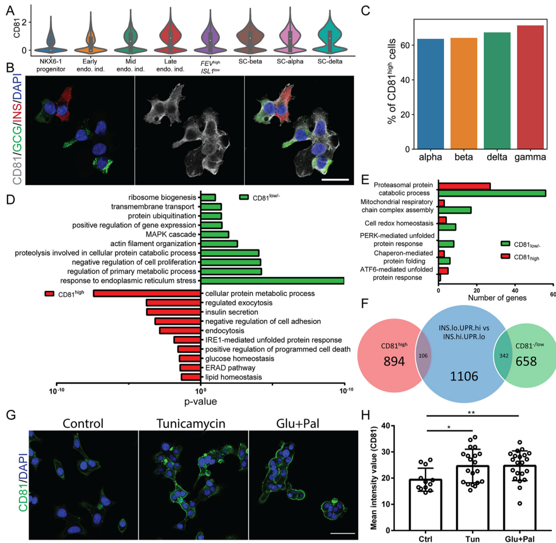
Figure 6: CD81 expression patterns in healthy and stressed human \beta -cells. (A) Violin plots indicating CD81 expression levels in different pancreatic cells during in vitro differentiation of endocrine cells from iPSCs. (B) Immunostaining of CD81 expression in stage (S) 6 of human endocrine cells derived from iPSCs. Scale bar 20 \mu m. (C) Bar plot showing the percentage of CD81 high cells in different endocrine cell types using scRNA-seq of healthy adult human islets. (D) GO-terms enrichment analysis for differentially regulated genes of human CD81 high and CD81 low \beta -cells. (E) Targeted analysis of specific signaling pathways related to ER stress coping mechanisms differentially regulated between human CD81 high and CD81 low \beta -cells. (F) Venn diagram showing a comparison between differentially expressed genes of human CD81 high and CD81 low \beta -cells with \beta -cell clusters described in Xin et al., 2018. (G) Immunostaining for CD81 (green) in control and treated Endo- \beta H1 cells. Scale bar 40 \mu m. (H) Quantification of the intensity levels of CD81 staining in Endo- \beta H1 cells (2 independent experiments; * P < 0.05; ** P < 0.01; t-test).
