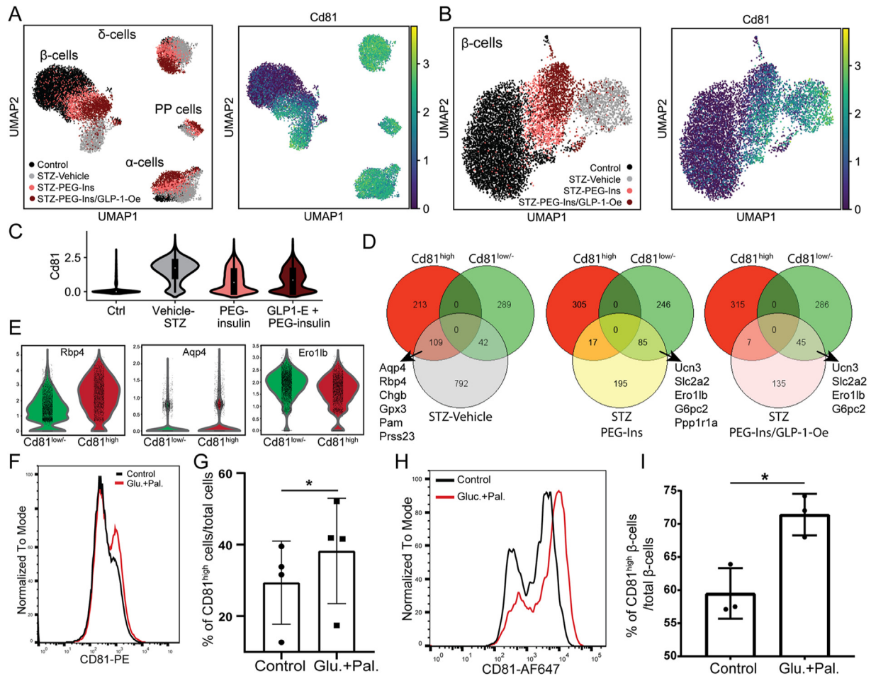
Figure 5: CD81 levels increased in stressed \beta -cells. (A) The left UMAP represents the different endocrine populations in control and treated animals. The right UMAP indicates the expression levels of Cd81 in different endocrine cell types from different treatments. (B) The left UMAP shows \beta -cell clusters in control and treated animals. The right UMAP displays the expression levels of Cd81 in \beta -cells from different treatments. (C) Violin plots representing Cd81 expression levels in \beta -cells among the different treatments. (D) Venn diagrams showing the comparison between differentially expressed genes of P16 Cd81 high and Cd81 low/- \beta -cells with differentially expressed genes in \beta -cells from STZ, STZ treated with PEG-Ins, and STZ treated with PEG-Ins/GLP-1-Oe. The analyses indicated in A–D were performed from the database described in Sachs et al., 2020. (E) Violin plots of representative genes upregulated ( Rbp4 and Aqp4 ) or downregulated ( Ero11b ) in P16 Cd81 high compared to Cd81 low/- \beta -cells. Rbp4 and Aqp4 were differentially upregulated in STZ \beta -cells. Ero11b was differentially upregulated in \beta -cells from STZ treated with PEG-Ins and PEG-Ins/GLP-1-Oe. (F) Histogram representing FACS analysis of CD81 expression levels in control and glucose+palmitate (Glu.+Pal.)-treated Min6 cells. (G) Quantification of FACS analysis indicating increased CD81 levels in stressed Min6 cells compared to controls (* P < 0.05; t-test). (H) Histogram showing FACS analysis of CD81 expression levels in control and Glu./Pal.-treated primary \beta -cells isolated from Nkx6-1-VF adult islets. (I) Quantification of FACS analysis revealing an increase in CD81 levels in stressed primary Nkx6-1-VF-derived \beta -cells (* P < 0.05; t-test).
