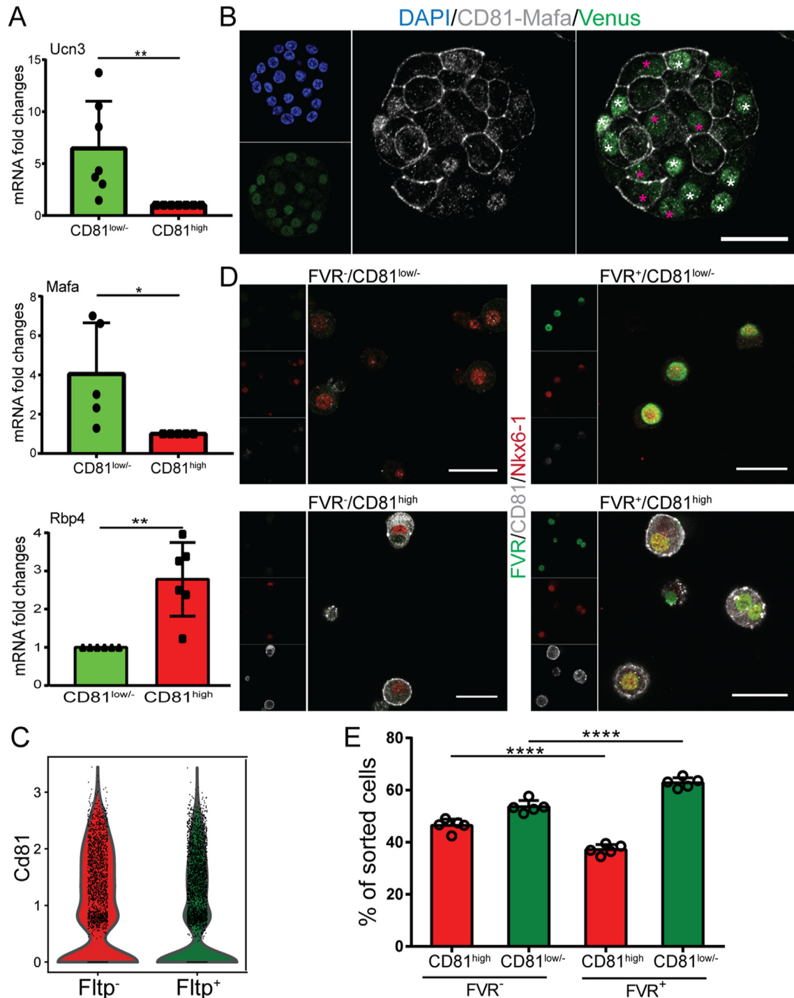
Figure 4: CD81 as immature \beta -cell markers. (A) qPCR analysis of maturation markers Ucn3 and Mafa and immature marker Rbp4 in sorted CD81 high and CD81 low/- \beta -cells isolated from Nkx6-1-VF mice (*P < 0.05; **P < 0.01; t-test). (B) Immunostaining of dispersed islet cells from P21 Nkx6-1-VF mice. Pink asterisks indicate Mafa - \beta -cells and white asterisks show Mafa + \beta -cells. CD81 and Mafa were imaged with the same confocal channel. Scale bar 20 \mu m. (C) Violin plots representing Cd81 expression levels in Fltp - and Fltp + \beta -cells at P16. (D) Immunostaining of sorted islet cells from adult Fltp-Venus reporter (FVR) mice based on FVR and CD81 expression levels indicating the presence of four different subpopulations: FVR - /CD81 low/- , FVR - /CD81 high , FVR + /CD81 low/- , and FVR + /CD81 high . Scale bar 50 \mu m. (E) Quantification of FAC-sorted cells indicating the number of FVR + and FVR - cells in CD81 high (left) and CD81 low/- (right) \beta -cell populations. (***P < 0.001; t-test).
