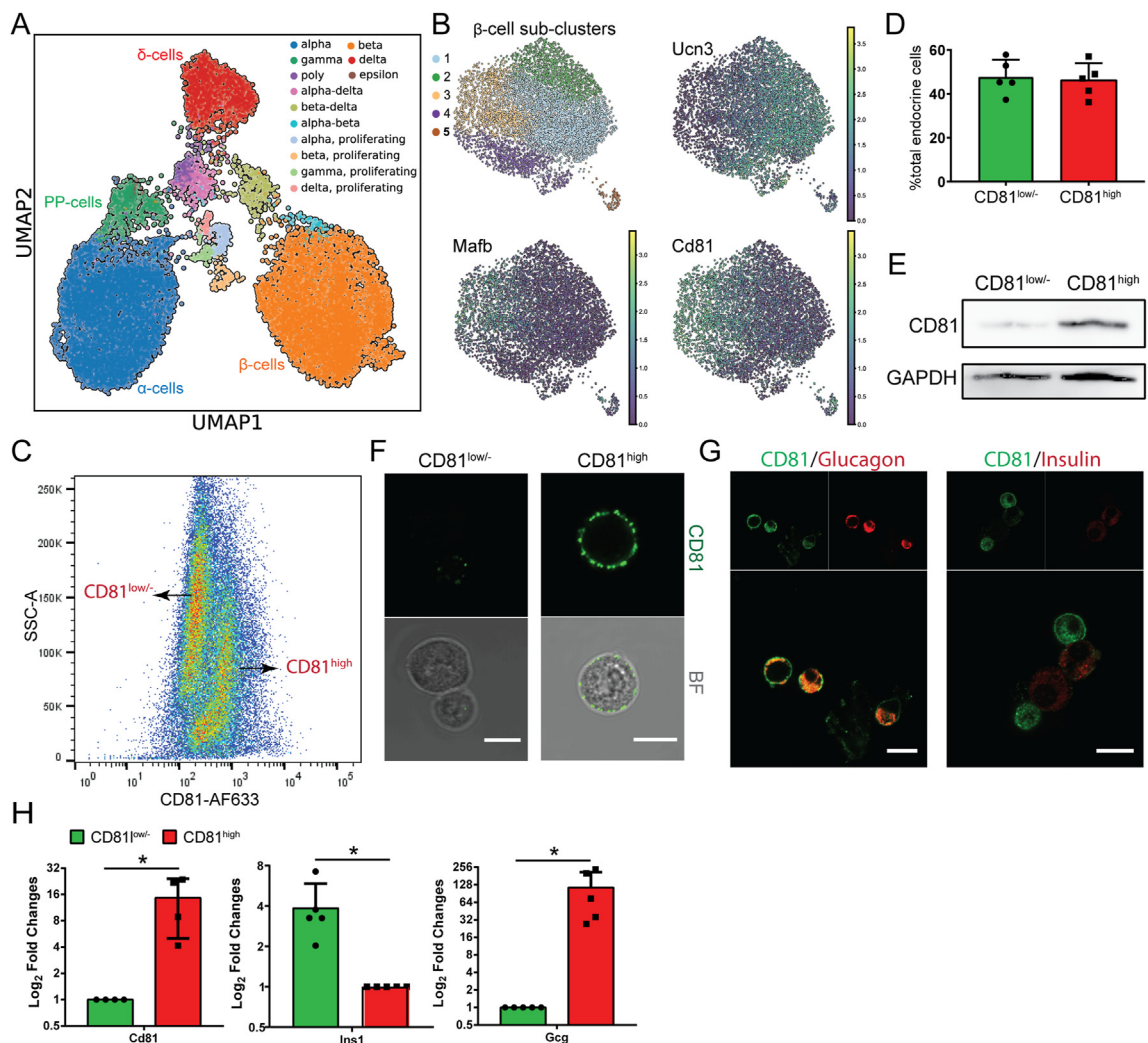
Figure 1: CD81 divided \beta -cells into two distinct subpopulations. (A) UMAP of 18,716 single cells from isolated islets from P16 mice. Different colors mark distinct endocrine cell types annotated based on the expression of signature hormone genes. (B) UMAPs representing only the \beta -cell cluster (7,275 single cells). On the top left, color-coded \beta -cell sub-clusters (1–5) identified by stochastic clustering (Louvain). The other 3 UMAPs indicate the mRNA expression levels (the lighter the color, the higher the expression) of Ucn3 , Mafk , and Cd81 in \beta -cells. (C) Representative FACS plot of adult mouse isolated islets stained for CD81. (D) Quantification of CD81 high and CD81 low/- adult endocrine cells by FACS analysis. (E) Representative Western blotting image from sorted CD81 high and CD81 low/- endocrine cells. (F) Representative confocal pictures of single endocrine cells right after sorting. Scale bar 10 \mu m. (G) Immunostaining for insulin (Ins), glucagon (Gcg), and CD81 on dispersed islets. Scale bar 10 \mu m. (H) qPCR analysis of CD81-based sorted adult endocrine cells (* P < 0.05 ; t-test).
