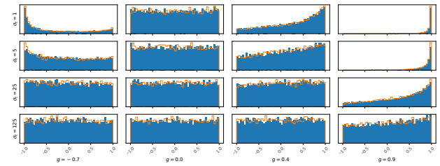
(a) Distribution of \cos(\theta) .
