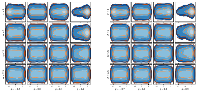
(b) Distribution of \alpha (vertical axis) as a function of \cos(\theta) (horizontal axis).
