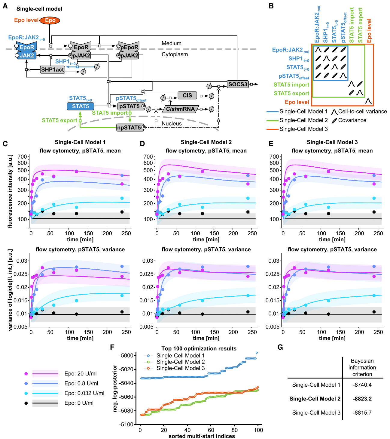
Figure 4. Dynamic mathematical JAK2/STAT5 pathway model describing cell-to-cell variability of phosphorylated STAT5 (A) The structure of the single-cell model of the JAK2/STAT5 pathway with putative sources of cell-to-cell variability of pSTAT5 (colored corresponding to the different models). (B) Visualization of covariance matrix for the three candidate models. (C–E) Experimental data (mean and variance of pSTAT5 from flow cytometry) and mixed-effect model outputs. See Figure S4 for correlation of data and model output and Figure S5 for full flow cytometry dataset and model output. (F) Multi-start optimization results for candidate single-cell models. Best 100 of 400 local optimization runs are shown, and plateaus indicate convergence. (G) Bayesian information criterion (BIC) values of the three candidate models.
