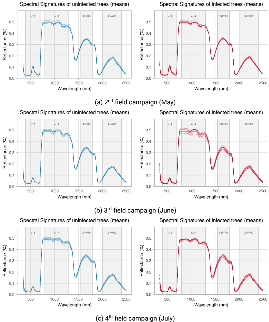
Figure 5.1: Uninfected (blue) and infected (red) tree respective mean leaf spectral signatures of all field campaigns
