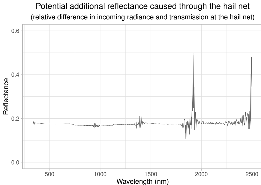
Figure 4.16: Potential additional reflectance caused through the hail net
