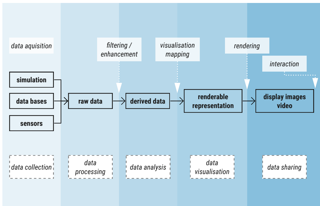
Figure 3.1: Visualisation Pipeline Scheme (based on Haber and McNabb, 1990)
