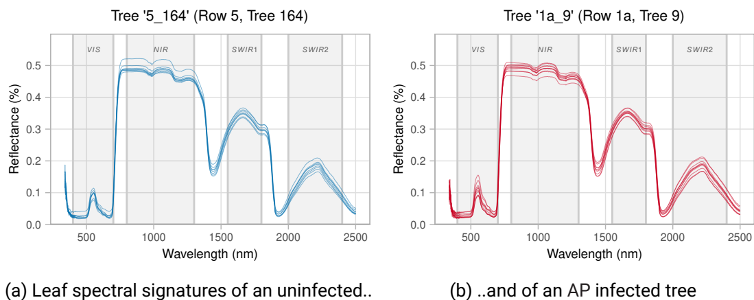
Figure 4.17: Comparison of Spectral Signatures of (a) an uninfected and (b) AP infected tree sampled in the second field campaign
