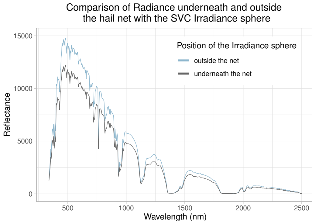
Figure 4.15: Comparison of Radiance underneath and outside the hail net with the SVC Irradiance sphere
