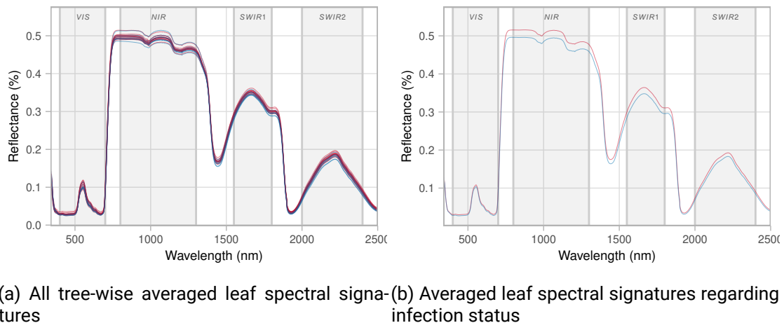
Figure 4.19: Leaf spectral signatures averaged (a) tree-wise and (b) regarding infection status sampled from the second field campaign
