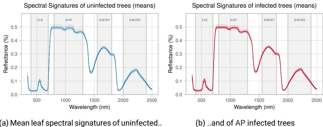
Figure 4.18: Comparison of mean spectral signatures of (a) uninfected and (b) AP infected trees sampled in the second field campaign
