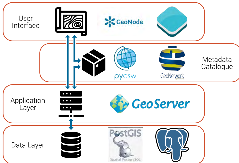
Figure 4.21: Spatial Data Schema used for the Implementation of the Precision map
