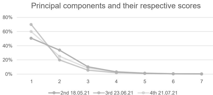
Figure 4.20: Scree plot of the PC's loadings regarding the entire hyperspectral range and from all field campaigns
