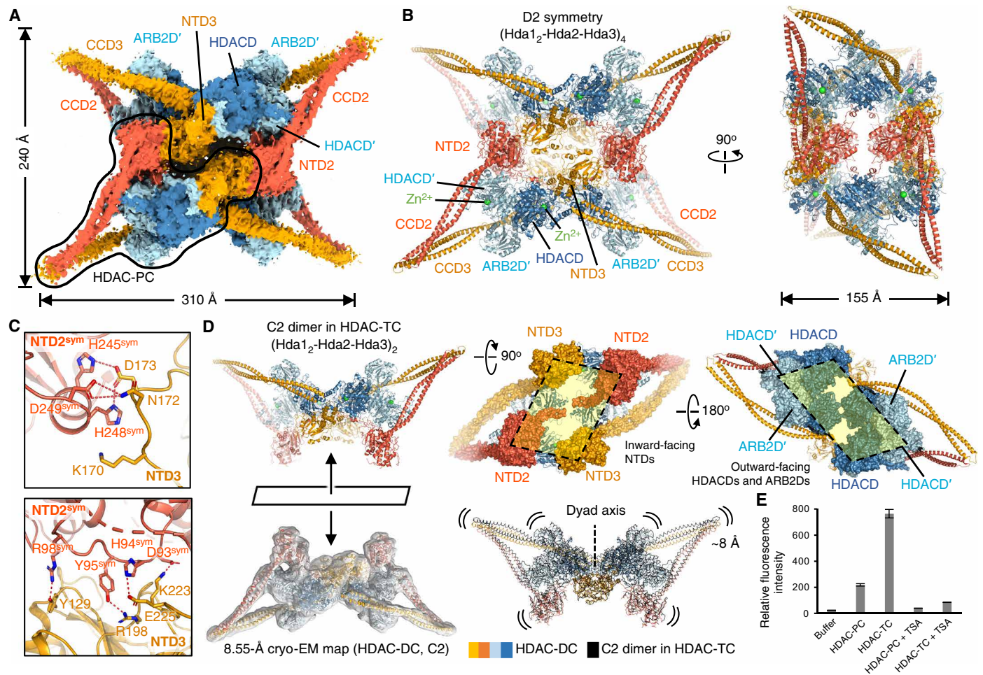
Fig. 5. The higher-order assembly is a nucleosome binding-deficient HDAC complex. (A) Cryo-EM map of the 1.3-MDa HDAC-TC at a resolution of 3.80 Å. (B) Two orthogonal views of a cartoon representation of HDAC-TC. (C) Magnified views showing tetramerization interfaces between NTD3 and C2 symmetry-related NTD2 (NTD2 sym ). The HDAC-TC structure was built by rigid-body fitting of four high-resolution structures of the HDAC-PC followed by PHENIX real-space refinement. (D) Quaternary structure (left) and subunit distribution (top right and middle) of HDAC-TC and overlay of HDAC-DC with C2 dimer observed in the halves of HDAC-TC (bottom center). (E) In vitro deacetylase activities of purified HDAC complexes with and without TSA. The assay was performed in triplicate, and the error bars are the SD of the data ( n = 3 ).
