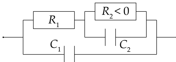
Fig. 10: Equivalent circuit fitted to the spectra in Figure 9. It fits the simulated spectra quite well, but for the measured spectra it neglects the 'kink' at around 0.2Hz and it does not describe the complex phase at \omega \rightarrow \infty .
