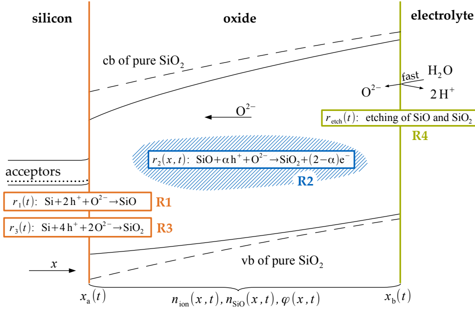
Fig. 2: A sketched band diagram of the model described in Section 3 with all the variables that define a state: Interface positions x_a(t) and x_b(t) , concentration of \text{O}^{2-} ions n_{\text{ion}}(x,t) , concentration of intermediate oxide n_{\text{SiO}}(x,t) and electric potential \varphi(x,t) . The bandgap of \text{SiO}_x (solid black line) is smaller than that of pure \text{SiO}_2 (dashed black line) [30]. Furthermore, the reaction that allows \text{O}^{2-} to enter the oxide layer is assumed to be fast compared to the transport inside the layer, so that the chemical potential of \text{O}^{2-} at x_b(t) is prescribed by the electrolyte.
