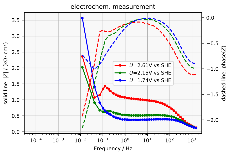
(b) Bode plot from the experimental data of Figure 7b.
