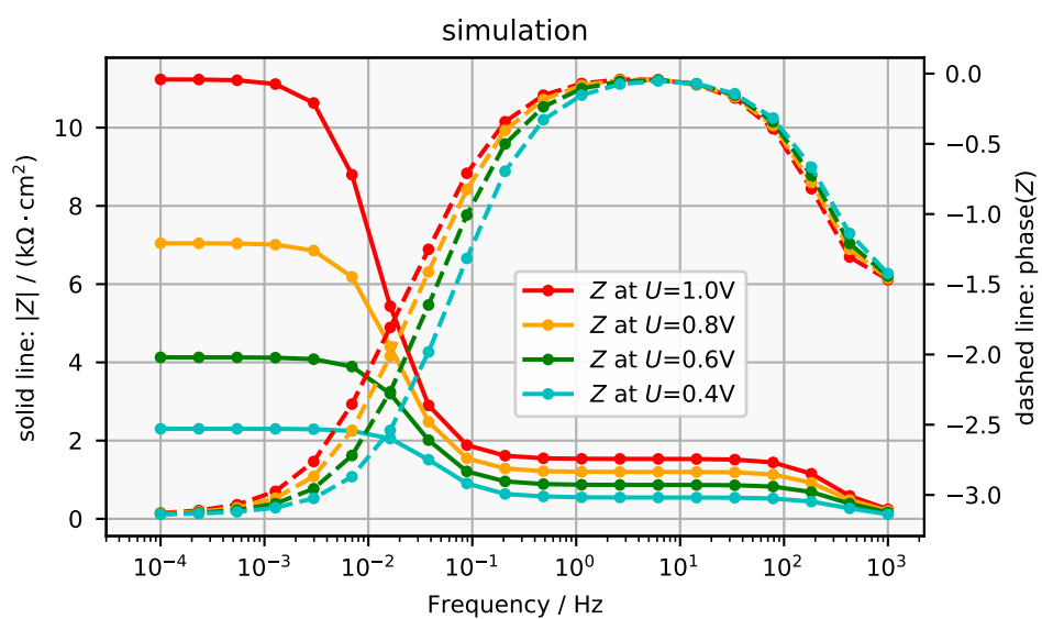
(a) Bode plot from the simulated data of Figure 7a.
