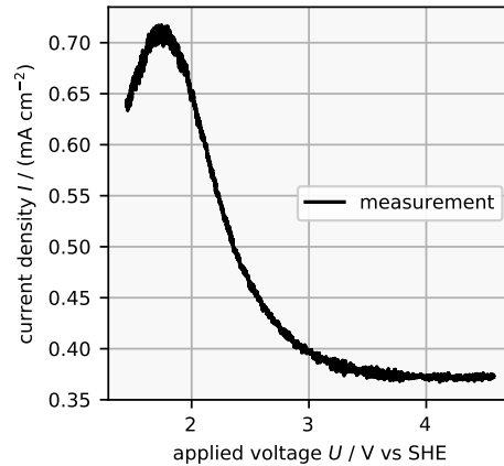
Fig. 1: 1 mV/s cyclic voltammogram of a (111) p-silicon electrode of 5 to 25 \Omega cm in a solution of 0.05 M \text{NH}_4\text{F} and 0.025 M \text{H}_2\text{SO}_4 (pH 2.3)
