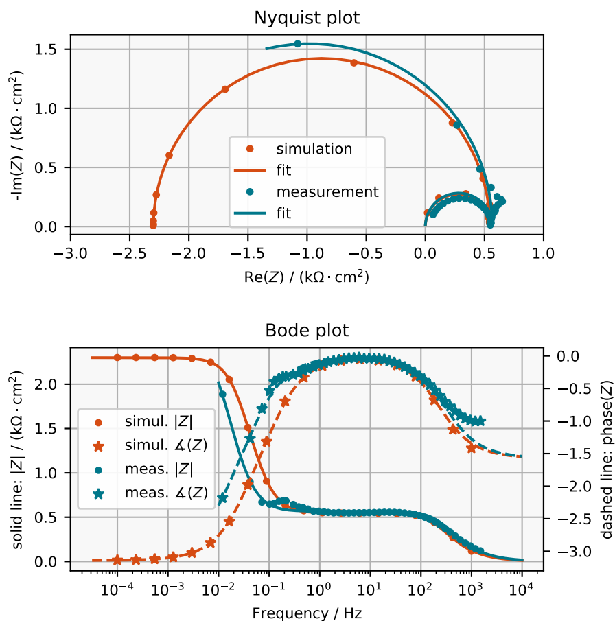
Fig. 9: One simulated impedance spectrum at voltage U = 0.4\text{V} and one measured impedance spectrum at voltage U = 2.2\text{V} vs SHE are exemplarily compared. Fits are represented by solid lines for the absolute value |Z| and by dashed lines for the complex phase of Z . The equivalent circuit can be seen in Figure 10. The circuits fit the simulated spectrum well but do not reflect all features of the measurement. These features become more/less dominant at higher/lower voltage, as can be seen in Figure 7b
