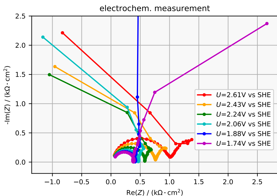
(b) This Nyquist plot shows impedance spectra that were measured with dynamic multi frequency analysis [27] for (111) p-silicon of 5 to 25 \Omega cm in a solution of 0.05M \text{NH}_4\text{F} and 0.025M \text{H}_2\text{SO}_4 (pH2.3).
