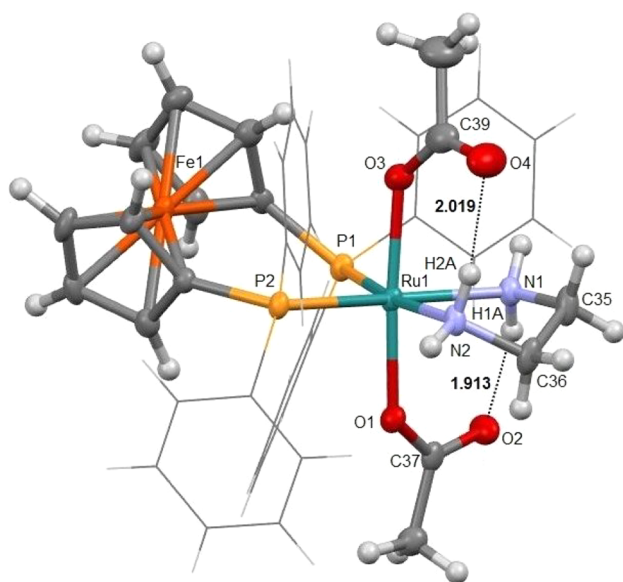
Figure 1. ORTEP style plot of compound 7 in the solid state (CCDC 2058063). Ellipsoids are drawn at the 50% probability level. The phenyl groups are simplified as wireframes for clarity (as well as disorder of one phenyl group is not shown). Selected bond lengths (Å) and angles (deg): Ru1–O1 2.109(3), Ru1–O3 2.118(3), Ru1–N1 2.164(4), Ru1–N2 2.155(3), Ru1–P1 2.2934(11), Ru1–P2 2.2816(11), O1–Ru1–O3 174.90(10), O1–Ru1–N2 87.73(13), O3–Ru1–N2 92.89(13), O1–Ru1–N1 89.91(13), O3–Ru1–N1 85.28(13), N2–Ru1–N1 77.99(13), O1–Ru1–P2 92.37(8), O3–Ru1–P2 92.69(8), N2–Ru1–P2 89.74(9), N1–Ru1–P2 167.42(10), N2–Ru1–P2 89.74(9), N1–Ru1–P2 167.42(10), O1–Ru1–P1 95.44(8), O3–Ru1–P1 83.23(8), N2–Ru1–P1 171.04(10), N1–Ru1–P1 93.61(10), P2–Ru1–P1 98.48(4). Hydrogen-bond distances measured for O2...H1A and O4...H2A are 1.913 and 2.019 Å, respectively.
