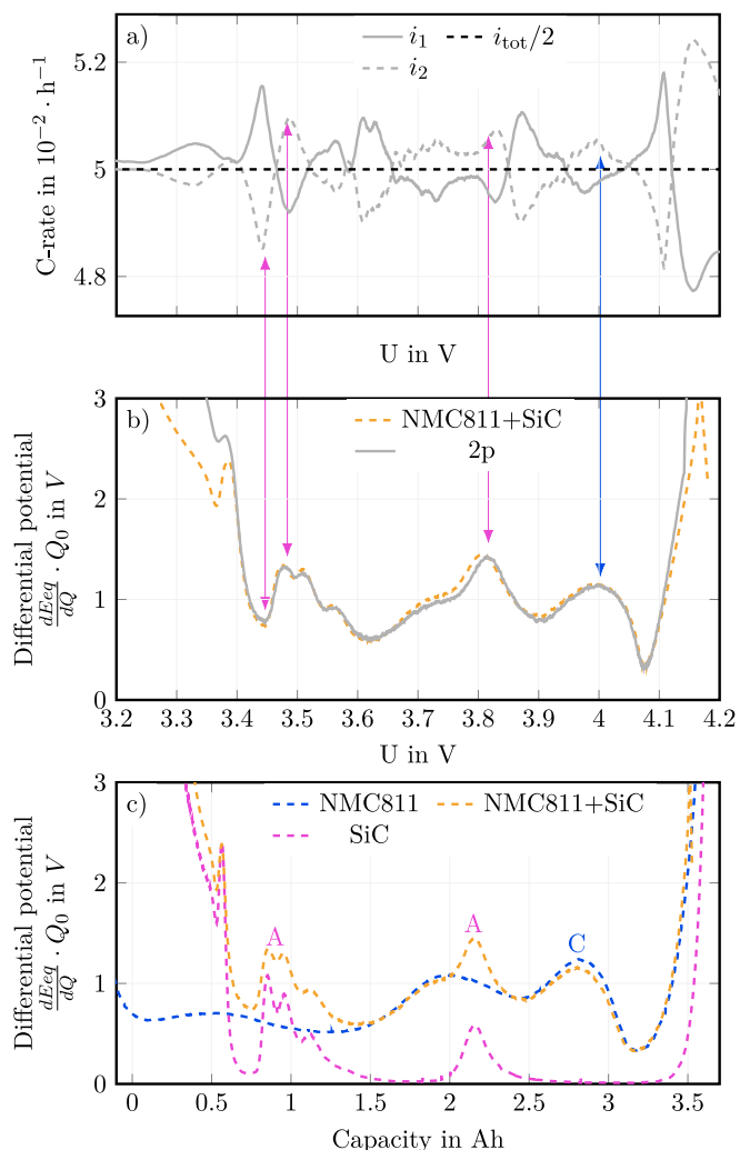
Fig. 8. Analysis of the DVA with the current distribution. (a) shows the current distribution between two parallel-connected cells with a homogeneous current in each branch of 0.05C. The corresponding DVA during the 2p measurement is shown in (b). Additionally, the dashed lines in (b) and (c) were extracted from [53] and correspond to the half cell profiles and full cells of this cell type with assigned characteristic material markers. The arrows show some areas where the local minima and maxima between the current i_2 and DVA appear on the same voltage level. (For interpretation of the references to colour in this figure legend, the reader is referred to the web version of this article.)
