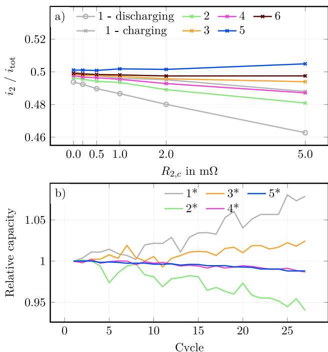
Fig. 7. Analysis of minima and maxima as well as intersection points of both currents. (a) shows the current spread at different points within different additional resistances due to an inhomogeneous load of Fig. 5. (b) shows the relative progress of intersection points of both currents according to Fig. 6 over all cycles within the investigation of homogeneous resistance in aspect to the loaded charge. (For interpretation of the references to colour in this figure legend, the reader is referred to the web version of this article.)
