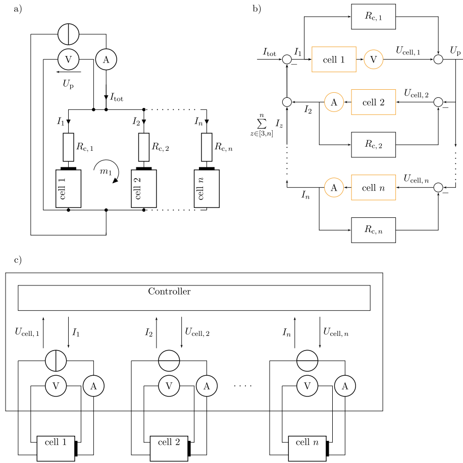
Fig. 1. (a) Simple ECM of a conventional n-parallel connection using a battery cycler in CC mode – current source and voltage measurement – in which each cell represents both the cell and its internal resistance, and a contact resistance, R_c that stands for any additional potential drop due to contacting, wiring and measurement equipment. (b) Closed-loop control system of a virtual n-parallel connection. The forward-path corresponds to the cell 1 with the additional resistance R_{c,1} and the feedback-path is equivalent to the cell 2 (cell n) with the additional resistance R_{c,2} ( R_{c,n} ). All symbols with an orange border refer to physical components. (c) Schematic of the virtual parallel connection within a n-channel battery cycler and physical cells connected to individuals channels via 4-wire technique. The controller calculates the setpoint of any channel with regard to Eqs. (1) and (3). Cell 1 is fed by a current source, see Eq. (1); current I_1 is the setpoint and voltage U_{cell,1} is the feedback parameter. All other n-1 cells are operated with a voltage source, see Eq. (3). Voltage U_{cell,n} is the setpoint and current I_n is the feedback parameter. (For interpretation of the references to colour in this figure legend, the reader is referred to the web version of this article.)
