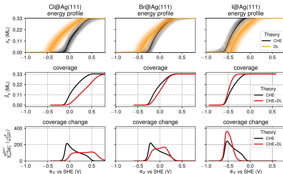
Figure 4. Analysis of the coverage-dependent contribution to the CVs in Figure 3. (Top) 2D energy landscape for the CHE excess energy ( g_{\text{exc},0}^{\theta_a, \text{CHE}} - T_{\text{S}_{\text{conf}}}^{\theta_a} ; black) and the DL term ( g_{\text{exc}}^{\theta_a, \text{DL}} , orange) (cf. eq 9). The solid lines follow the extremal value at fixed \Phi_E , while the diffuse range indicates the energy contour up to \pm 5 meV/site for the convex (concave) CHE (DL) energy profile. (Middle) Equilibrium surface coverage \bar{\theta}_a as extracted from the 2D energy landscape. At the CHE level (black line); this is simply the extremal ridge shown as a black line in the top panel. At the CHE + DL level (red line), this is the extremal ridge of the 2D landscape resulting after summing the CHE and DL contributions. (Bottom) Area-normalized derivative \frac{d}{d\Phi_E} \bar{\theta}_a / A_{\text{site}} determining the coverage-dependent contribution to the CV peak shape (see text).
