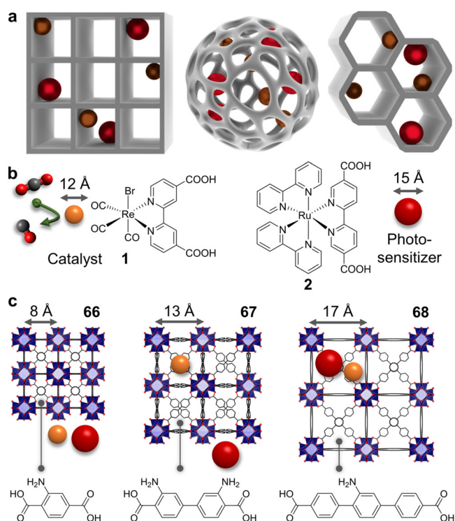
Figure 1. a) Representation of integrated molecular photosystems (spheres) in various assembly-controlling MOF topologies. b) Structures of CO 2 reduction catalyst [ReBr(CO) 3 (4,4'-dcbpy)] ( 1 ) and photosensitizer [Ru(bpy) 2 (5,5'-dcbpy)]Cl 2 ( 2 ). c) Anchoring sites of 1 and 2 in the isoreticular UiO ( 66 , 67 , 68 ) host series based on pore sizes and the respective MOF linkers.
