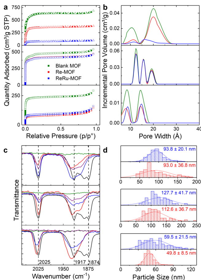
Figure 3. Assembly characterization. 66 (bottom), 67 (middle), 68 (top) with pristine MOFs (green), Re-MOF (red), ReRu-66 (R MOF 2.7, blue), ReRu-67 (R MOF 0.4, blue), ReRu-68 (R MOF 2.0, blue), and corresponding post-catalysis ReRu-MOFs (purple). a) N 2 adsorption isotherms at 77 K. b) Calculated pore size distributions. c) ATR-IR spectra from 1810 to 2075 cm -1 of MOF assemblies and pure 1 (black). d) Particle size histograms from SEM. Bottom to top: Re-66 , ReRu-66 (R MOF 2.7), Re-67 , ReRu-67 (R MOF 0.4), Re-68 , ReRu-68 (R MOF 2.0).
