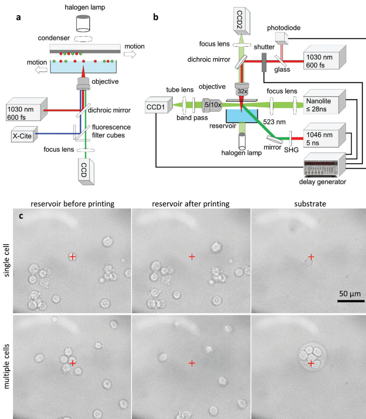
Figure 1. Laser-based transfer of single cells and of cell clusters. a) Laser-based cell-transfer setup combined with inverted optical microscopy for cell selection. b) Upright optical configuration, as used for time-resolved analysis of the transfer process shown in Figures 2a,c and 3e, and in Figures S1, S2, and S7, Supporting Information. c) Single (upper panel) and multiple (lower panel) B16F1 cells are identified with an optical microscope (bright field, 32× objective, NA = 0.6), selected and transferred from a hydrogel reservoir to a target substrate. Red crosses mark the center of the bright field images, which correspond to the laser focus position in the reservoir (left images). The laser pulse energy is 3 μJ and the focus depth is 70 μm. Scale bar for all micrographs = 50 μm.
