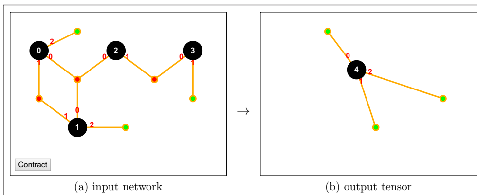
Figure 3: Illustration of an elementary contraction operation.
