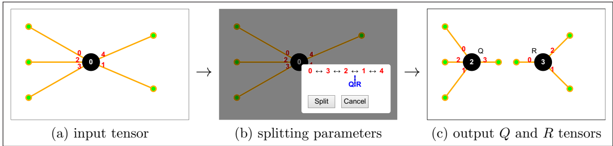
Figure 4: QR splitting of a tensor. In (b) , the user specifies the ordered dimensions attributed to the Q and R tensors, respectively.
