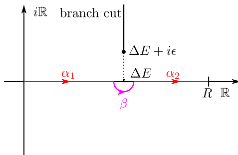
Figure 11. Contour used to compute the vacuum part. Black dot: the pole of the function G_\epsilon ; \alpha_1 , \alpha_2 : paths on the real line; \beta : path in the complex plane (half circle) avoiding the singularities of G_\epsilon .
