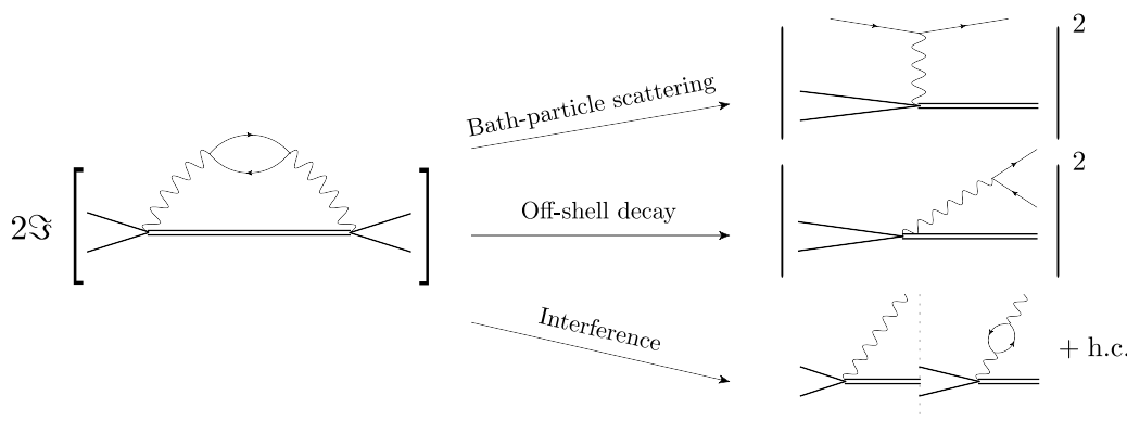
Figure 4. Diagram shows contributions contained in the photon spectral function at next-to-leading order.
