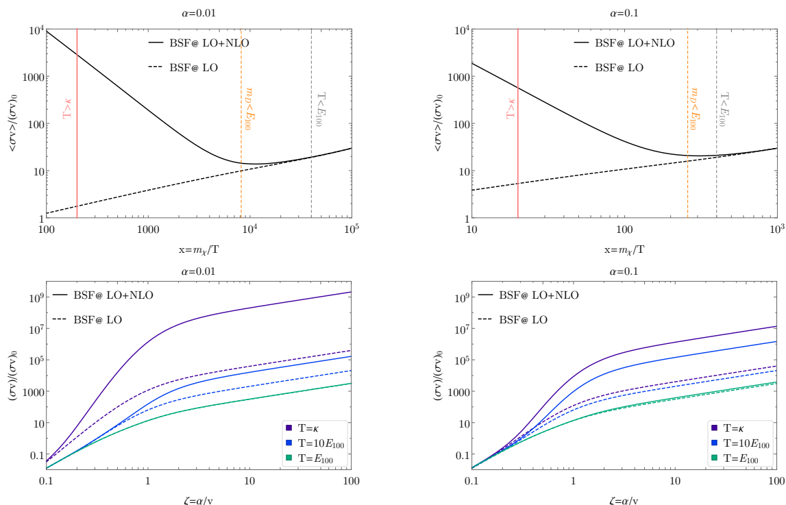
Figure 5. Lower row shows the bound-state formation cross sections. Upper row compares the thermally averaged quantities. The cross sections are normalized to (\sigma v)_0 \equiv \pi\alpha^2/m_\chi^2 . From left to right, the vertical lines indicate when temperature is larger than the Bohr momentum \kappa = \mu\alpha , the electric Debye mass m_D^2 = g^2T^2/3 and the temperature are smaller than the ground state binding energy.
