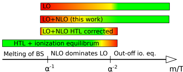
Figure 10. Illustration of the goodness of different descriptions, based on the assumption that the mediator is (unsuppressed) coupled to the primordial plasma background. LO and LO+NLO indicate bound-state formation via LO emission of an on-shell mediator only or including higher order contributions to the photon spectral function, respectively. The bottom bar represents HTL resummed corrections to the Sommerfeld enhanced annihilation and bound-state decay rate under the assumption of ionization equilibrium.
