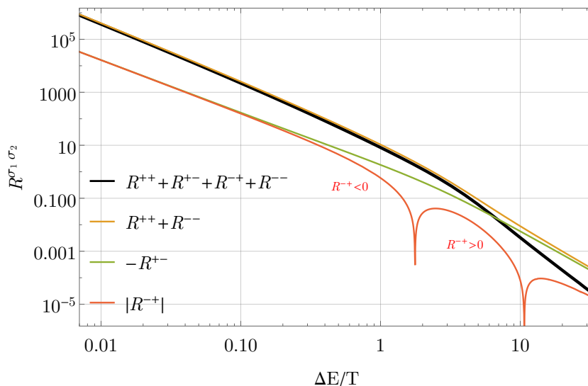
Figure 14. The plot shows the individual R^{\sigma_1 \sigma_2} functions and their dependence on \Delta E/T .
