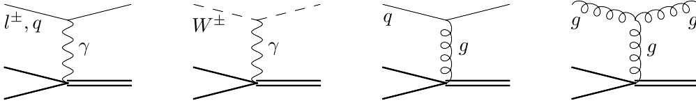
Figure 1. Graphic shows electrically or color charged coannihilation examples where bound states are formed via bath-particle scattering. The amplitudes for these processes are divergent in the forward scattering direction of the bath particles. Parallel black solid lines represent the bound state, while open lines correspond to the initial two-particle scattering state.
