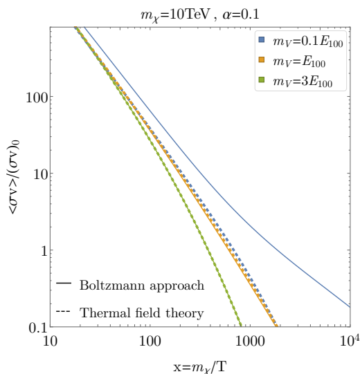
Figure 6. Comparison of the thermally averaged bound-state formation cross section for bath-particle scattering in the conventional Boltzmann and the thermal field theory approach.
