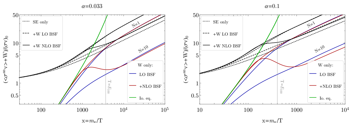
Figure 7. Importance of NLO BSF processes for different N . Upper (lower) solid and dashed black line, as well as upper (lower) red and blue line correspond to the N = 1 ( N = 10 ) case. All quantities are normalized to (\sigma v)_0 \equiv (1 + N) \pi \alpha^2 / m_\chi^2 , such that the curve for SE annihilation and for W in ionization equilibrium are independent of N .
