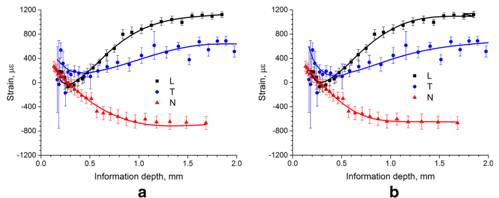
Fig. 8 Strain profiles along the BD-line of the welded plus machined sample for the three main directions: longitudinal, transverse, and normal. Points are the neutron diffraction measurements, and the lines are the fits obtained for a free model (a) and a model fixed to XRD values at the surface (b)
