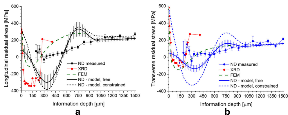
Fig. 11 Longitudinal (a) and transverse (b) residual stress profiles along the BD-line of the welded plus machined sample measured by x-ray and neutron diffraction. Comparisons with finite element modeling and neutron spurious strain corrections and data deconvolution within the gauge volume are as well pictured
