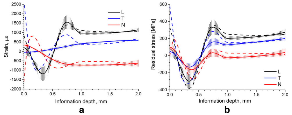
Fig. 9 Deconvoluted residual strain (a) and stress (b) profiles corresponding to the fits in Fig. 9, free model (solid lines) and constraint model fixed to the surface XRD value (dashed lines). The error bars indicate 1\sigma confidence limits estimated by the bootstrap method [35]
