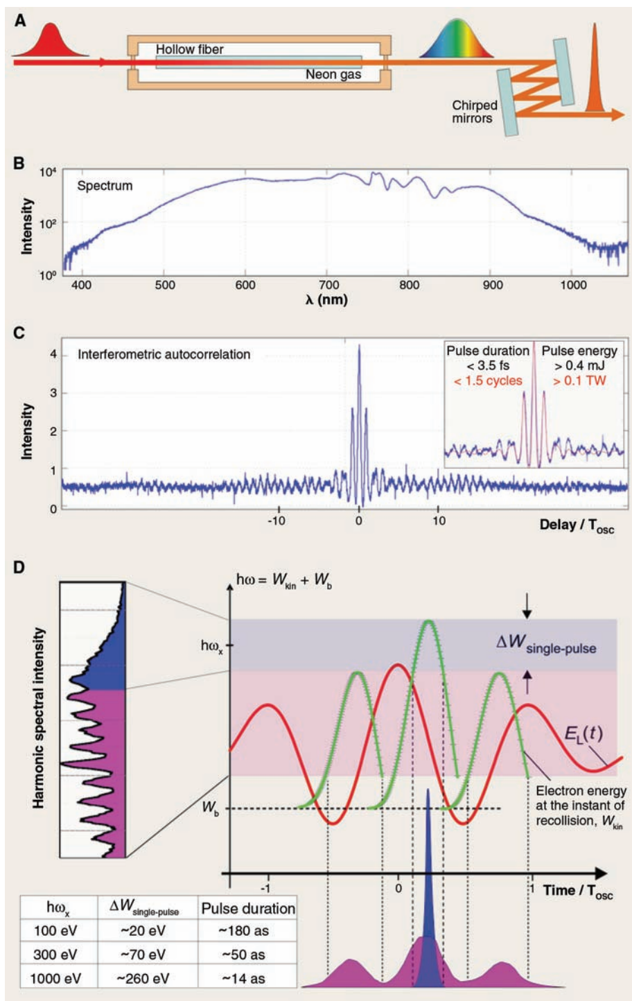
Fig. 3. Toward intense, monocycle optical pulses. (A) Hollow-fiber/chirped-mirror optical pulse compressor for the generation of intense, few-cycle laser pulses. (B) The spectrum of millijoule-energy, near-20-fs, phase-controlled near-infrared laser pulses delivered at a repetition rate of 3 kHz from a Ti:sapphire laser (Femtopower, Femtolasers GmbH) is first broadened to more than an octave ( \sim 450 to 950 nm) in a neon-filled capillary (pressure \sim 2 bar, length \sim 1 m, bore diameter 250 \mu\text{m} ). (C) The spectrally broadened pulses are compressed by octave-spanning chirped multilayer mirrors. The interferometric autocorrelation trace indicates a near-bandwidth-limited \sim 3.5 -fs pulse carried at \lambda_L \approx 720 nm. (D) Energies of XUV photons emitted from an atom exposed to a linearly polarized 3.5-fs, 720-nm Gaussian laser pulse that is sufficiently intense for efficient tunnel ionization. The photon energies (green lines) are depicted as a function of the return time of the electron to the atomic core and have been obtained by analyzing classical electron trajectories (43). The width of the energy band within which only one recollision contributes to XUV emission determines the bandwidth \Delta W_{\text{single-pulse}} available for the generation of an isolated attosecond pulse. Based on the classical trajectory analysis, \Delta W_{\text{single-pulse}} is found to be maximum for a near-cosine-shaped waveform, E_L(t) = E_0 \varepsilon(t) \cos(\omega_L t + \varphi) , with the carrier-envelope phase \varphi varying between \pi/12 and \pi/6 depending on the pulse shape and intensity. Here, E_0 and \omega_L stand for the amplitude and angular frequency of the oscillations of the laser electric field, with \varepsilon(t) being the amplitude envelope function. The table summarizes bandwidths over which the sub-1.5-cycle pulses are predicted to support the emergence of an isolated attosecond pulse at different XUV photon energies. The estimated pulse durations derive from the conservative assumption that no spectral components are available for the pulse synthesis outside the given spectral window.
