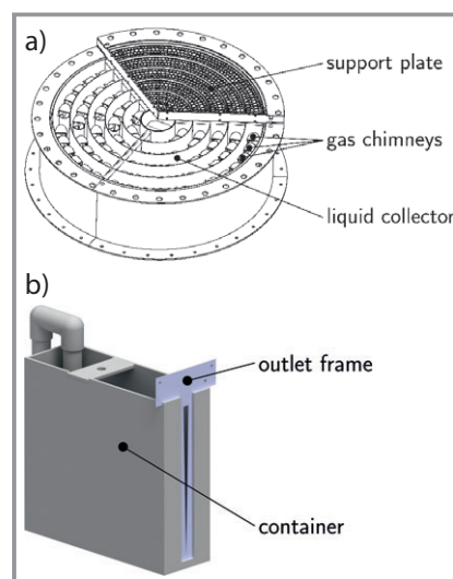
Figure 11. a) Liquid collector of the \text{\O} 1.2 \text{ m} packed column at TU Munich [25]. b) Measuring cell for determination of liquid flows [25].
