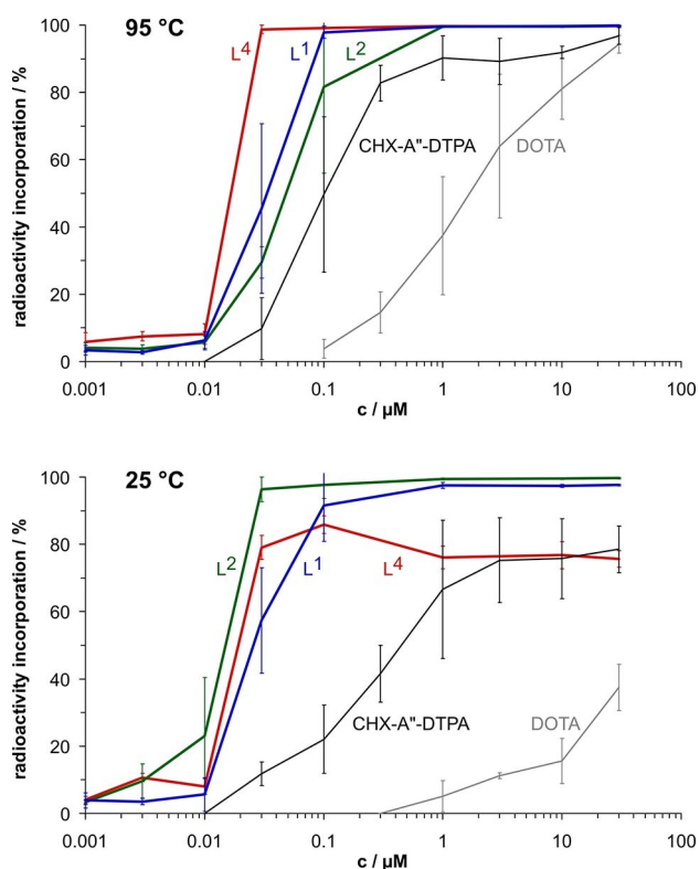
Figure 3. Incorporation of 213 Bi III by bispidine ligands L 1 , L 2 , and L 4 as a function of ligand concentration. Radiometal complexation was performed in a total volume of 0.1 mL at pH 5 for 5 min at 95 (top) and 25 °C (bottom); data are given as mean values ± SD, n = 3–6. Literature data for CHX-A''-DTPA and DOTA are shown for comparison. [5]
