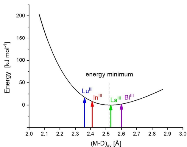
Figure 2. Hole size (and shape) curve for \text{L}^4 (adapted from ref. [21]). The strain energy (MOMEC program and force field [33–36] ) is plotted as a function of the averaged metal–donor distances (\text{M}-\text{D})_{\text{av}} with the minimum of the curve set to 0 \text{kJ mol}^{-1} . Apart from the metal–donor atom–ligand backbone angle deformation, the curve does not include any metal-ion-dependent terms. The variation of the metal–donor atom distances was asymmetric (i.e., the shape of the ligand and its variation were taken into account). The approximation adopted included full geometry optimization of the \text{Zn}^{\text{II}} complex as a large metal ion and the \text{Co}^{\text{III}} complex as a small metal ion and linear approximation between these structures to determine the relative changes in metal–donor atom distance for all eight bonds.
