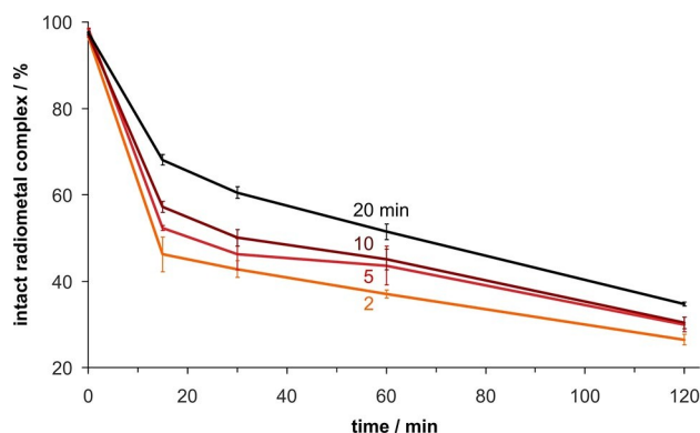
Figure 5. Percentage of intact ^{213}\text{Bi}^{\text{III}}\text{-L}^4 species as functions of time upon challenge with 0.1 M aqueous sodium DTPA (pH 7.5, 37 °C). Labeling prior to challenge was done at pH 5 and 25 °C for different durations (2, 5, 10, and 20 min); data are given as mean values \pm SD, n = 3 .
