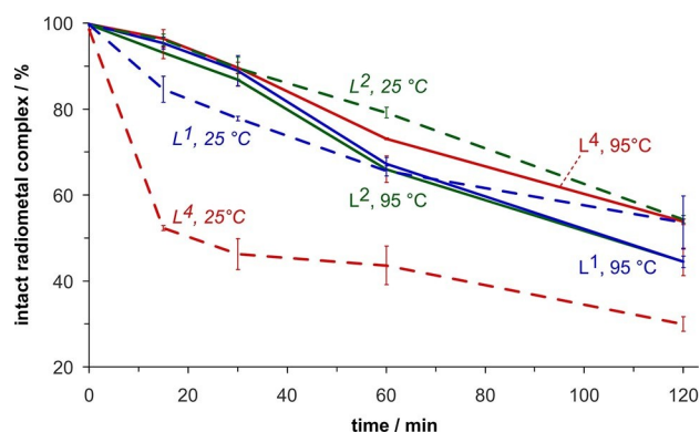
Figure 4. Percentage of intact 213 Bi III complexes as a function of time upon challenge with 0.1 M aqueous sodium DTPA (pH 7.5, 37 °C). Labeling prior to challenge was done at pH 5 for 5 min and either at 95 °C (solid lines, upright labels) or 25 °C (dashed lines, labels in italics); data are given as mean values ± SD, n = 3.
