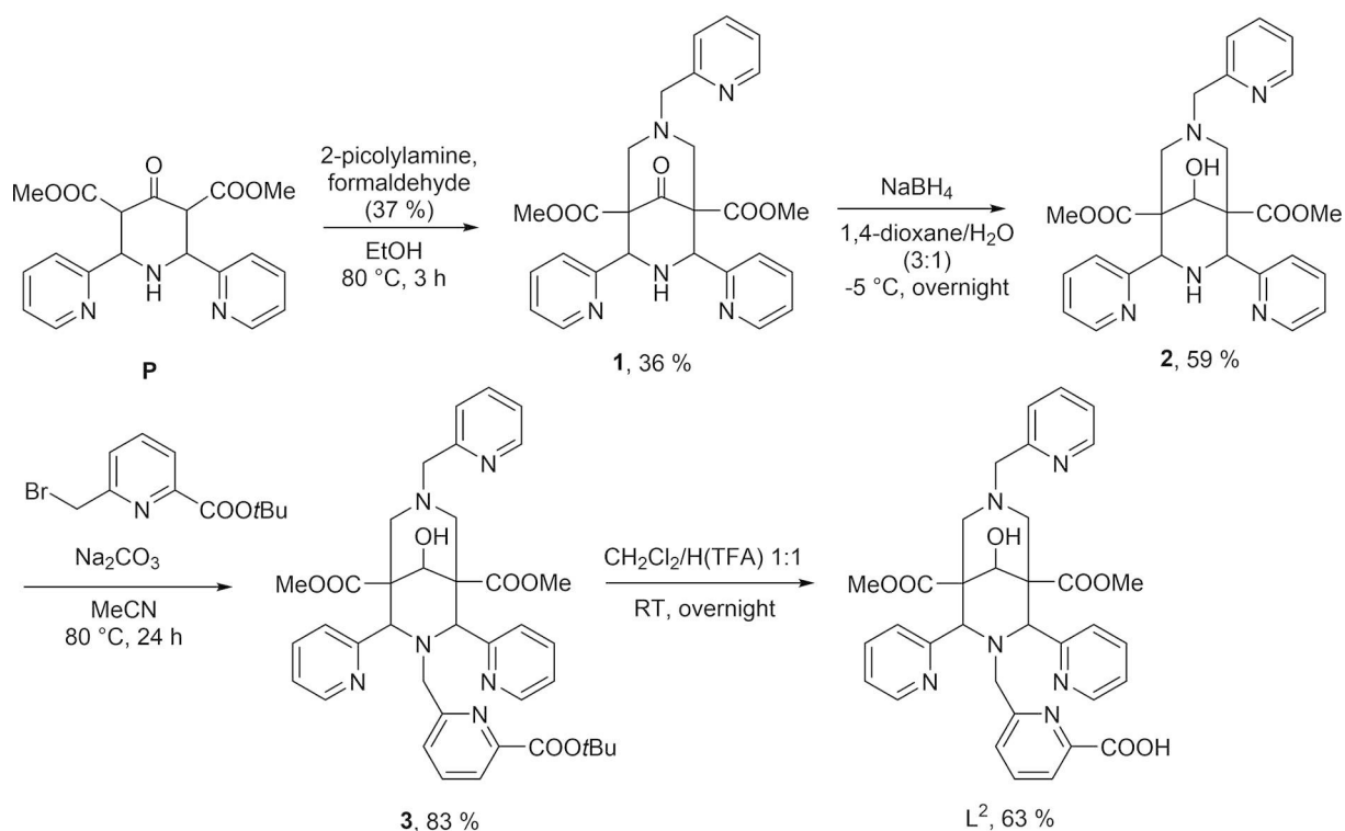
Scheme 1. Synthesis of L 2 .
