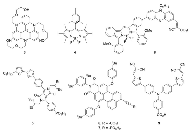
Figure 4. Organic PSs used in photocatalytic fuel synthesis.
