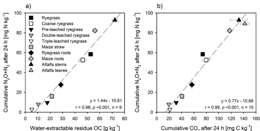
Fig. 3. Relationship between (a) water-extractable residue OC and cumulative \text{N}_2\text{O} + \text{N}_2 production after 24 h of anoxic incubation (except for alfalfa leaves because of \text{NO}_3^- depletion) as well as (b) between cumulative amounts of \text{CO}_2 and \text{N}_2\text{O} + \text{N}_2 at the end of incubation. Error bars represent standard deviation of means ( n = 3 ).
