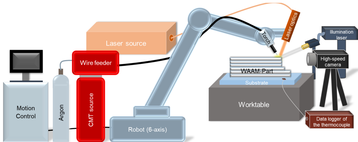
Fig. 1. Schematic experimental set-up of the robot based WAAM cell (Figure is for printing full size and in colour).
