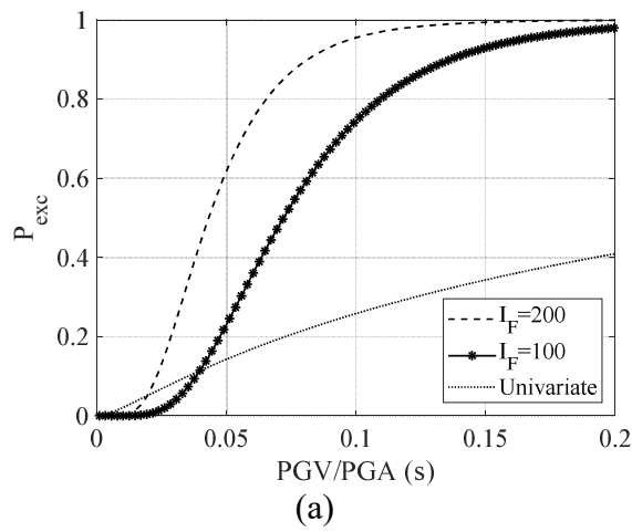
Figure 13: Bivariate and univariate fragility curves for moderate rocking (LS2) of smCHc: PGV/PGA for different IF values (a); PGA for different IF values (b).
