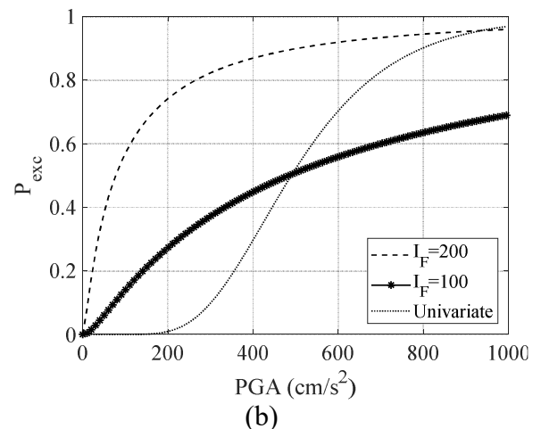
Figure 13: Bivariate and univariate fragility curves for moderate rocking (LS2) of smCHc: PGV/PGA for different IF values (a); PGA for different IF values (b).
