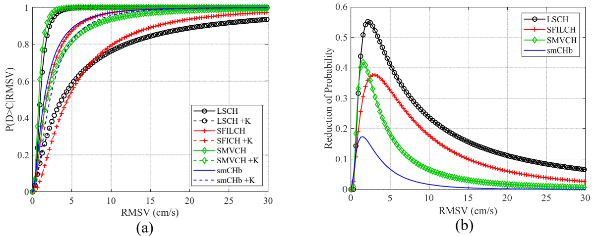
Figure 10: Univariate fragility curves for the yielding limit state with IM=RMSV: conditional probability (a) and reduction of probability (b) from the one-sided motion to the restrained one-sided motion.
