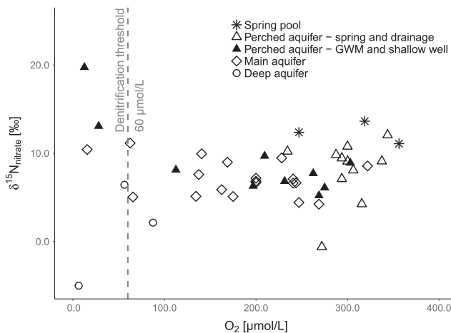
Figure 6. Plot of \delta^{15}\text{N}_{\text{nitrate}} against \text{O}_2 concentrations to determine potential denitrification; The \text{O}_2 threshold concentration of 60\ \mu\text{mol/L} has been drawn in with a dashed line.
