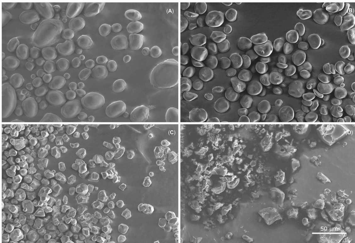
FIGURE 9 | Scanning electron microscope images show raw powders of potato starch (A), barley starch (B), corn starch (C), and protein (D). Different particle morphologies between the different starch powders are clearly visible. Potato starch particles are both round and elliptical with a very smooth surface, whereas barley starch consists of round and lenticular particles with fine cracks on the smooth surfaces. Corn starch forms polyhedral particles with rough surfaces. Protein shows no principal particle morphology and different surface roughnesses are visible.
