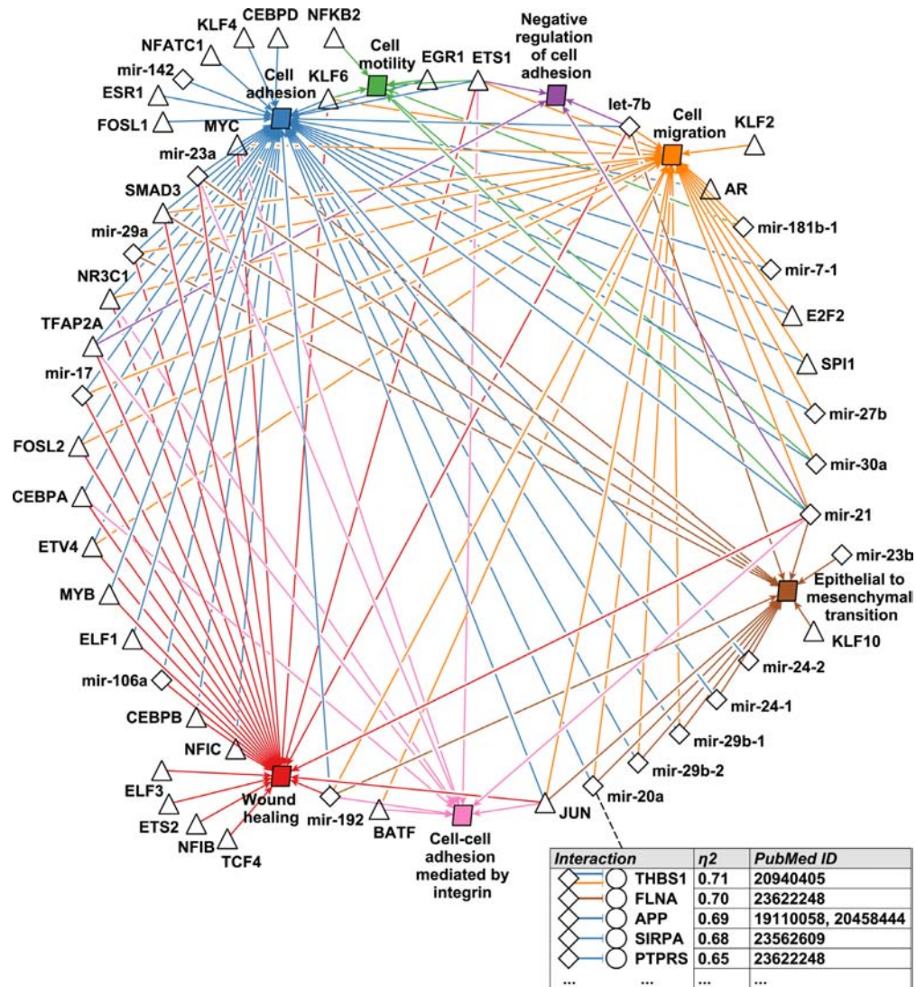
Figure 5. Metastatic interplay of TFs and miRNAs. Nodes are biological processes (colored parallelogram), TFs (triangle) and miRNAs (diamond). Arcs denote an enrichment of RG targets in a metastatic process and are colored, respectively. The top five predicted negative regulations of miR-20a are listed exemplary in the table shown at the lower right corner; e.g. the THBS1 repression by miR-20a which was described in (68) and holds a condition-specific regulation score of 0.71. This interaction affects cell adhesion and cell migration (blue and orange arcs). Note that the shown network was filtered by regulatory interactions having at least one literature reference (PubMed ID).
