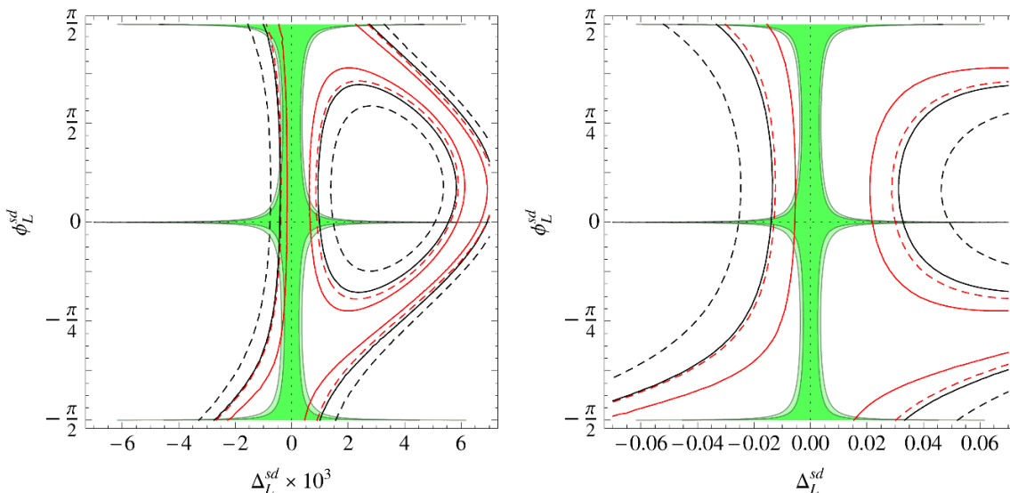
Figure 2. Prospects for observing new physics in K decays. The green regions show the 68% C.L. and 95% C.L. allowed regions in the \Delta F = 2 fit. The contours show the 3\sigma and 5\sigma projections for \mathcal{B}(K^+ \rightarrow \pi^+ \nu \bar{\nu}) in 2019 and 2024, the colours are as in figure 1. Left: M_{Z'} = 5 TeV and \Delta_L^{\nu\bar{\nu}} = 1 . Right: M_{Z'} = 50 TeV and \Delta_L^{\nu\bar{\nu}} = 3 .
