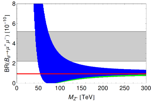
Figure 9. \mathcal{B}(B_d \rightarrow \mu^+ \mu^-) versus M_{Z'} in the L+R scenario. The red line corresponds to SM central value and grey area is the experimental region: (3.6_{-1.4}^{+1.6}) \times 10^{-10} .
