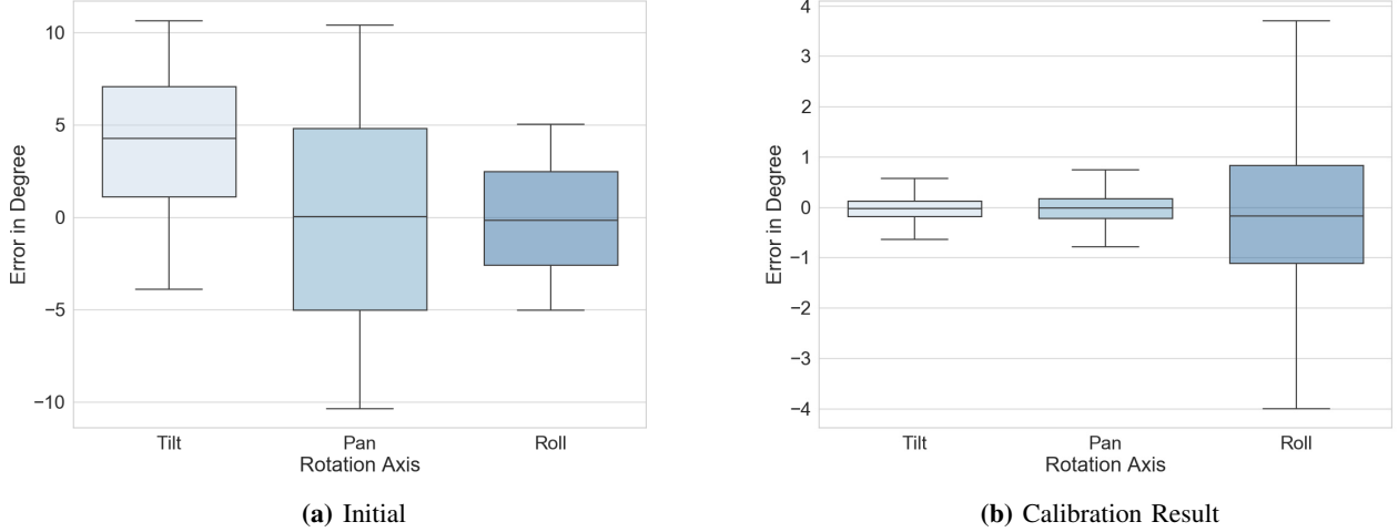
Fig. 4: Initial and resulting errors for each rotation angle on test set \mathcal{T}_1 with random calibration errors. Note that the positive shift for the tilt angle errors is a result of filtering the samples with less than 10 projected detections in the image, as described in Sec. V-A. Tilting the camera downwards likely moves the detections out of the upper image border.
