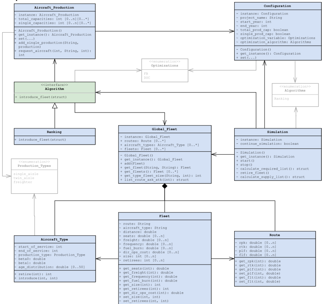
Fig. 9 – UML diagram of the object-oriented fleet model implementation
