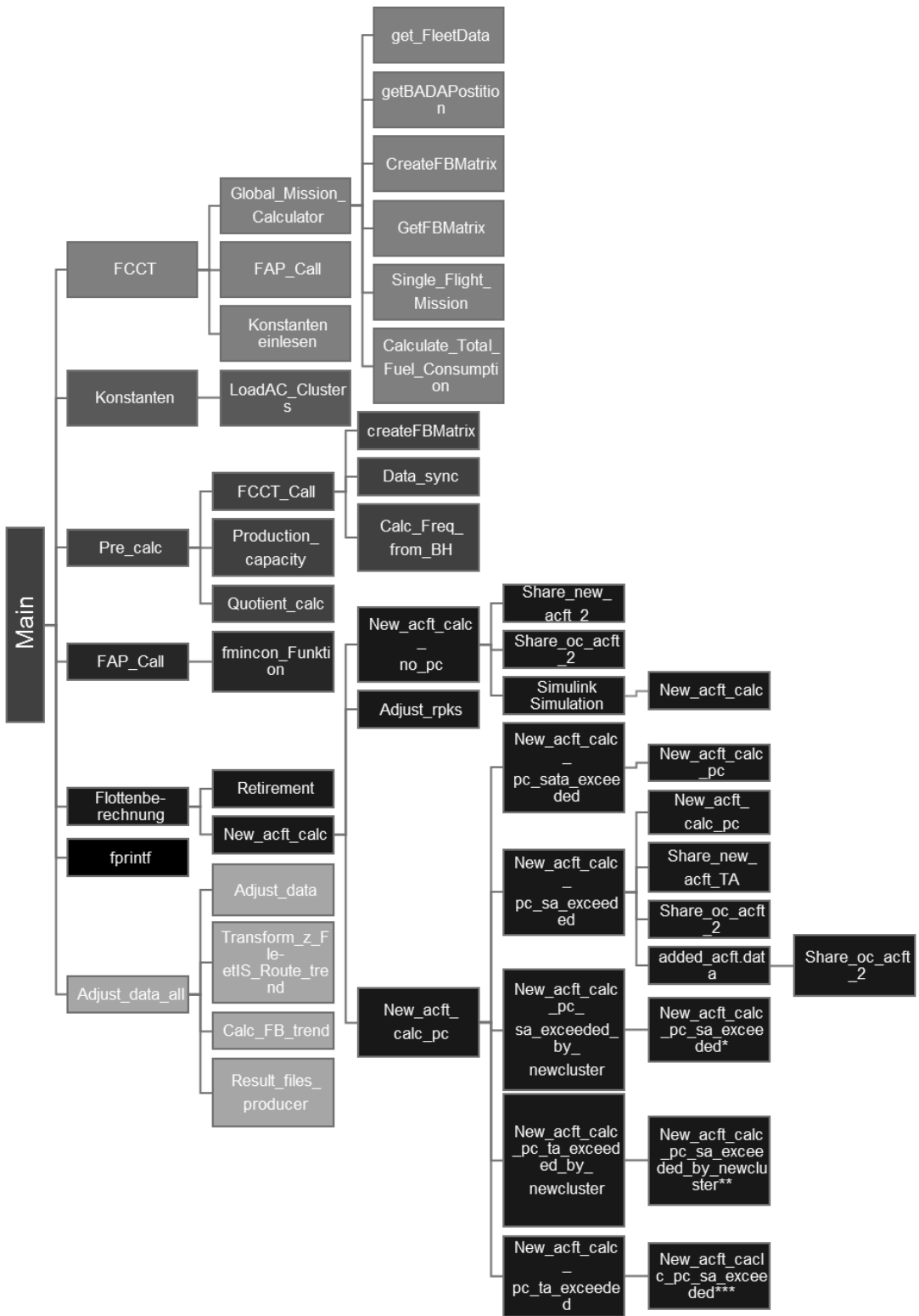
Fig. 5 – Basic structure of scripts in the non-object-oriented fleet model
