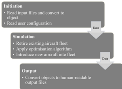
Fig. 7 – Macro phase structure of the object-oriented program.
