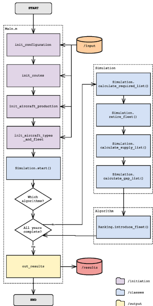
Fig. 8 – Flowchart of the object-oriented fleet model implementation
