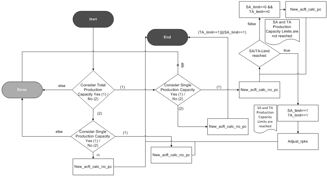
Fig. 6 – Flowchart of the script “New_acft_calc”
