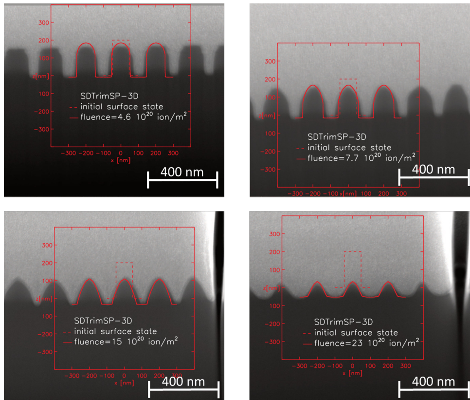
Figure 5.14: FIB-enabled cross-sections of the Si sample exposed under the (0^\circ, 0^\circ) scenario, imaged at various fluence steps. The solid red line denotes the cross-section of the target morphology generated by SDTrimSP-3D at the same fluence steps. The dashed red line indicates the cross-section of the initial target model used in the simulation.
