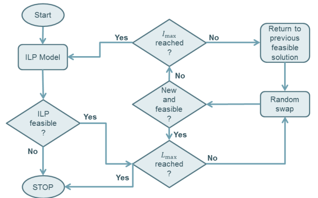
Fig. 1. Flow chart of the enumeration method.
