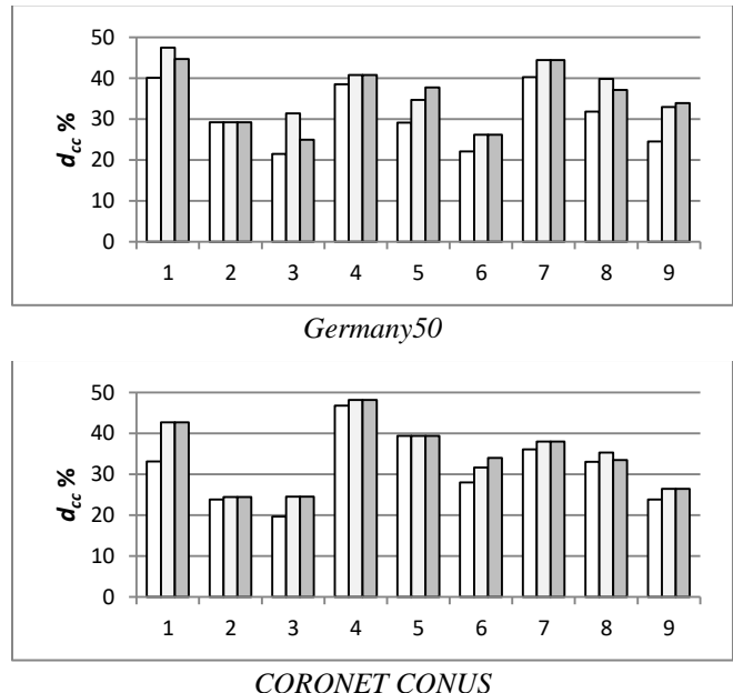
Fig. 5. Average CC delays of the MinAvgCC solutions (white columns), best robust CPP solutions against set M' (grey columns) and against set M (dark grey columns) for all instances of Germany50 (top) and CORONET CONUS (bottom).
