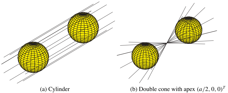
Fig. 1. Extreme situations of the set of hyperboloids for disjoint spheres
