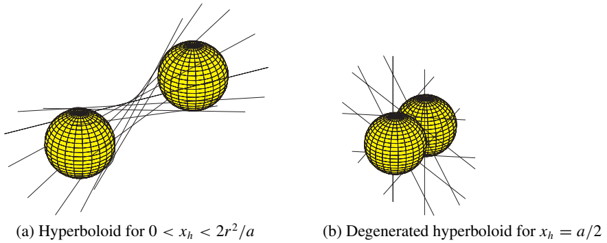
Fig. 2. The left figure shows a general situation for disjoint spheres; the right figure shows an extreme situation for non-disjoint spheres
