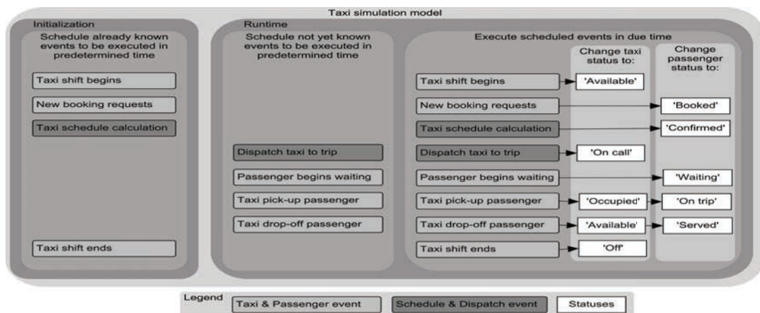
Fig. 4. Taxi simulation model features and structure.
