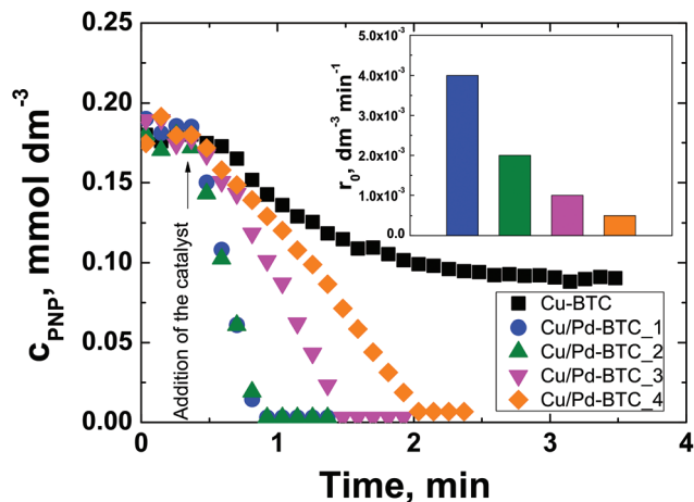
Fig. 3 Concentration of PNP as a function of time for non-doped Cu-BTC and Pd containing Cu/Pd-BTC_1–4 as catalysts in the aqueous-phase hydrogenation of PNP with NaBH 4 to PAP. The insert shows the initial reaction rate for Cu/Pd-BTC_1–4 normalized to the amount of Pd in the catalyst, respectively. Reaction conditions: C_{\text{PNP}} = 0.18 \text{ mmol dm}^{-3} , C_{\text{NaBH}_4} = 0.60 \text{ mmol dm}^{-3} , T = 298 \text{ K} , stirring speed = 1300 \text{ min}^{-1} , m_{\text{catalyst}} = 5.0 \text{ mg} , ambient pressure.
