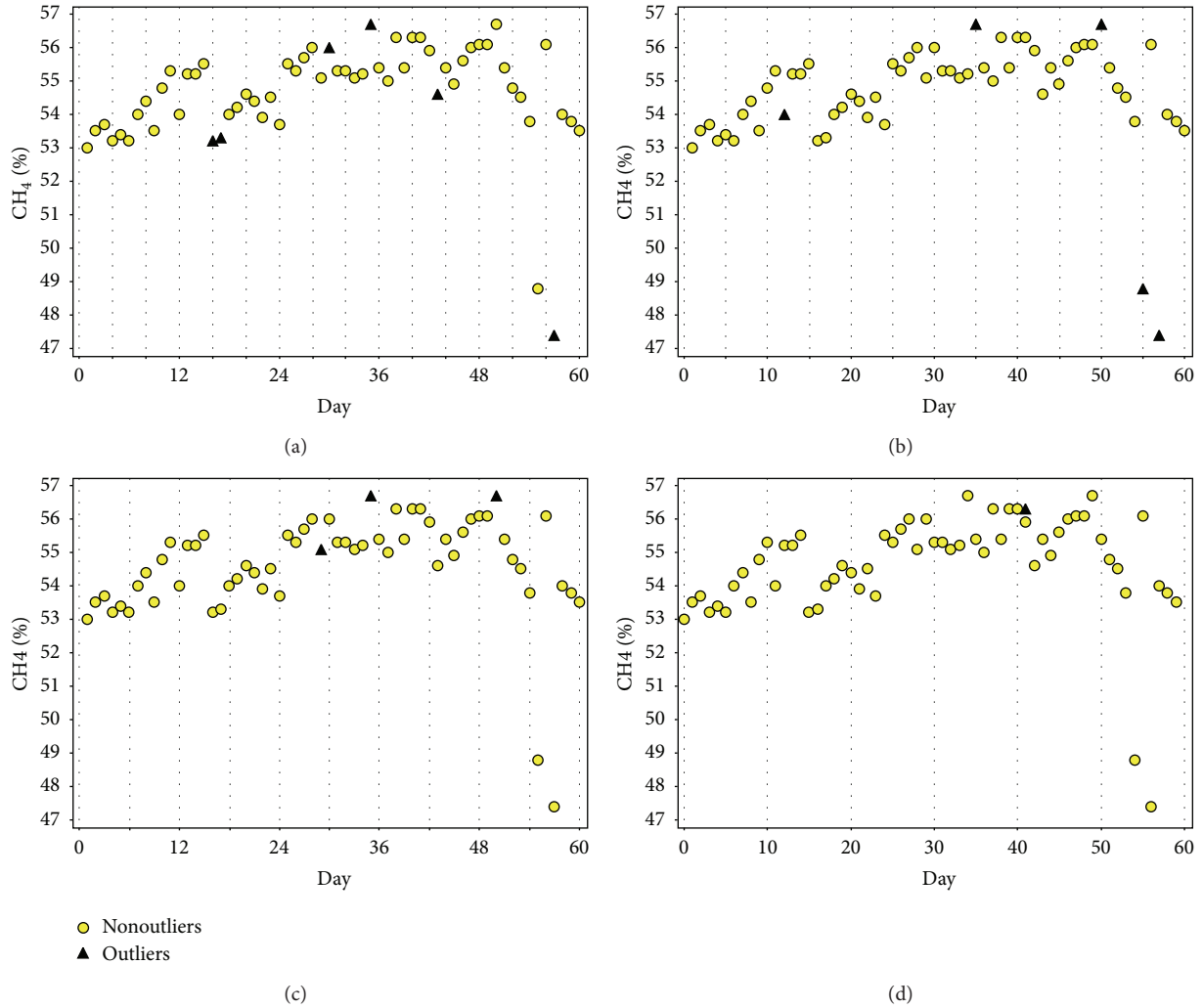
FIGURE 6: Outlier detection of volumetric percentage of CH4 in biogas with new transformation technique for significance level of 0.05 for different window sizes without overlap. Plots (a), (b), (c), and (d) correspond to window sizes 4, 5, 6, and 10, respectively.
