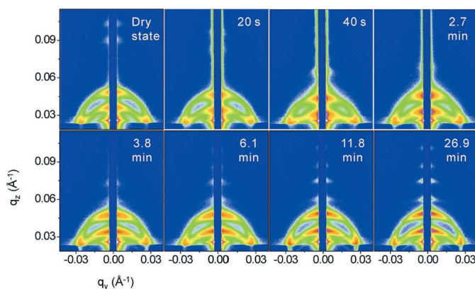
Figure 7 Two dimensional GISAXS data of a lamellar poly(styrene b butadiene) diblock copolymer film during the first swelling step at the times given. The logarithmic intensity scale runs from 10 to 7000 counts for all images. Reprinted with permission from Di et al. (2012). Copyright (2012) American Chemical Society.
