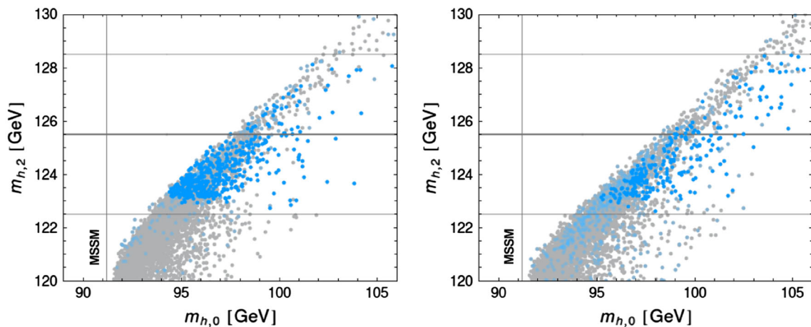
Fig. 5 The two-loop Higgs mass ( m_{h,2} ) as a function of the tree-level Higgs mass ( m_{h,0} ) for MI (left) and MII (right). Points satisfying all constraints for which m_{\tilde{t}_1} < 2 TeV are bright blue , paler points indicate low-energy constraints are satisfied and stop masses are in the range 2
