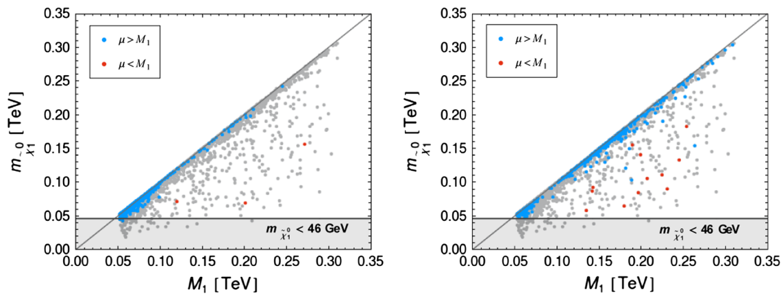
Fig. 8 The lightest neutralino mass ( m_{\tilde{\chi}_1^0} ) as a function of M_1 for MI (left) and MII (right). The grey points are excluded by experimental constraints. The grey diagonal line indicates m_{\tilde{\chi}_1^0} = M_1 , and the horizontal line indicates the LEP exclusion limit as described in the text
