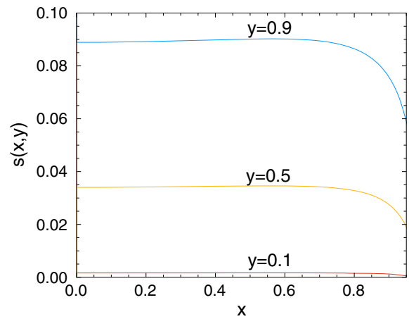
Fig. 10 We show s(x, y) as a function of the parameter x for fixed values of y as indicated
