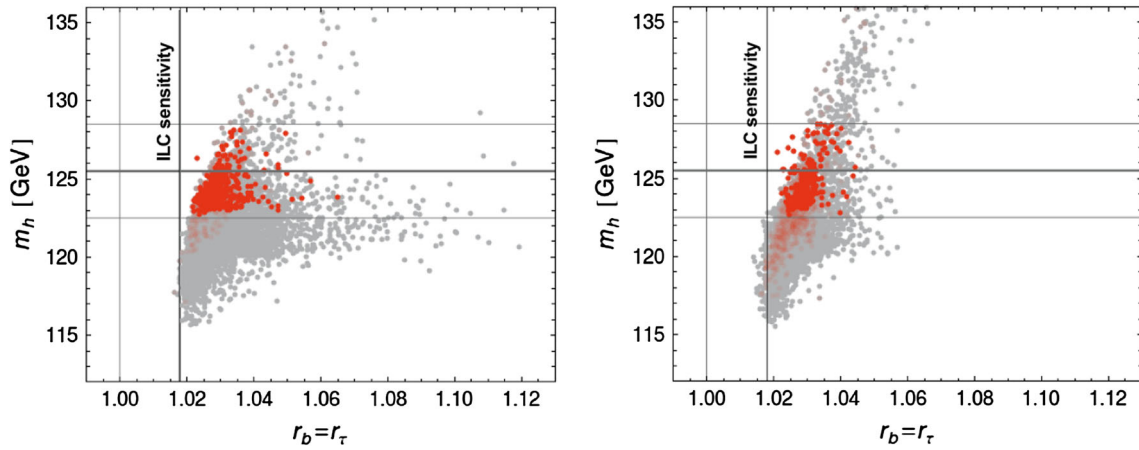
Fig. 6 The Higgs mass as a function of r_b = r_\tau for MI (left) and MII (right). Points satisfying all constraints and m_{\tilde{\tau}_1} < 2 TeV are bright red, whereas paler points indicate that stop masses are in the range 2 \text{ TeV} < m_{\tilde{\tau}_1} < 2.3 TeV and only low-energy constraints are satisfied.
