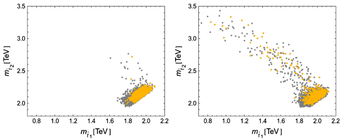
Fig. 3 The mass of the heavy stop m_{\tilde{t}_2} as a function of m_{\tilde{t}_1} for MI (left) and MII (right). Points satisfying low-energy and the Higgs mass constraints are shown in yellow, whereas the remaining excluded points are shown in grey
