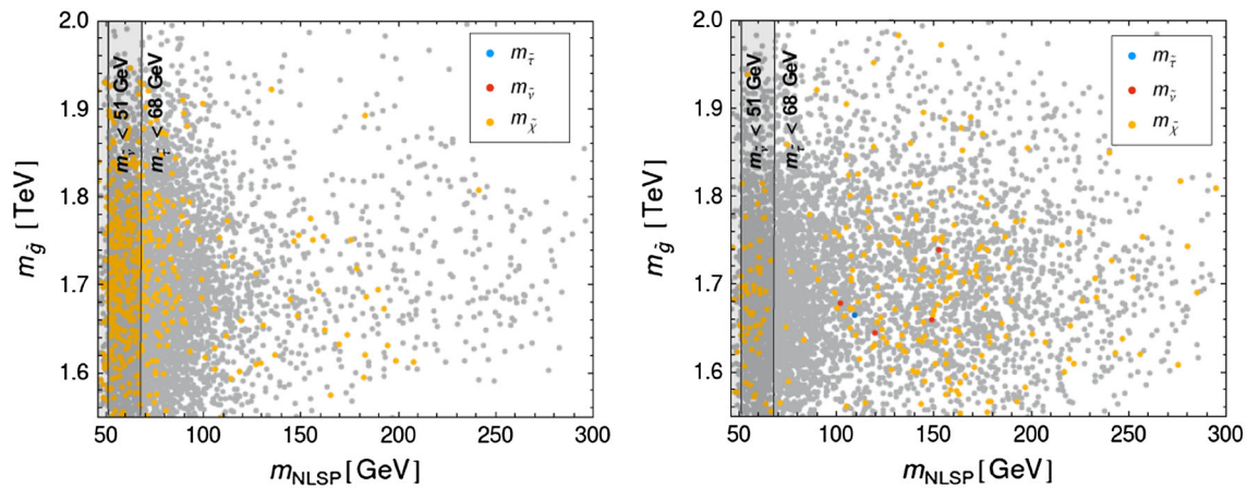
Fig. 7 The gluino mass ( m_{\tilde{g}} ) as a function of NLSP mass ( m_{\text{NLSP}} ) for MI (left) and MII (right), where the colours indicate the type of NLSP as shown in the legend. The LEP exclusion limit for the case of the \tilde{\tau}
