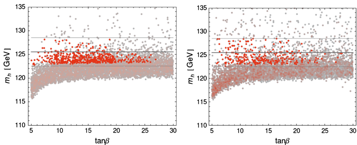
Fig. 4 The Higgs mass as a function of \tan\beta for MI (left) and MII (right). Points satisfying all constraints and m_{\tilde{t}_1} < 2 TeV are bright red, whereas paler points indicate that stop masses are in the range
