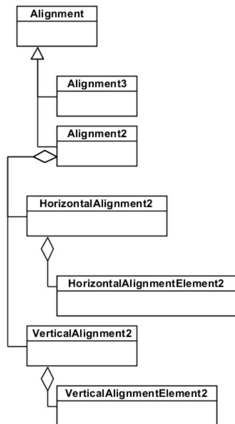
Figure 1. Top level view of the meta-alignment model.
