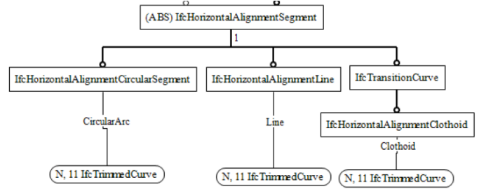
Figure 5. Horizontal alignment segments use and IfcTrimmedCurve (part of standard IFC 4) to describe its geometry
