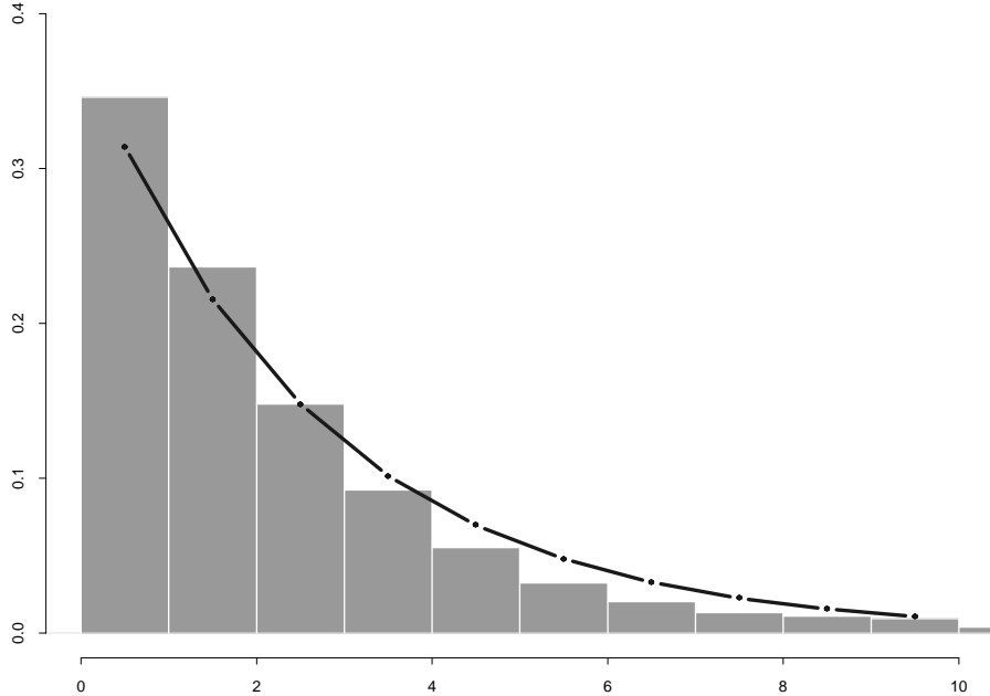
Figure 3: Histogram, corresponding to Table 4 with fitted density of truncated geometric distribution (4.20).
