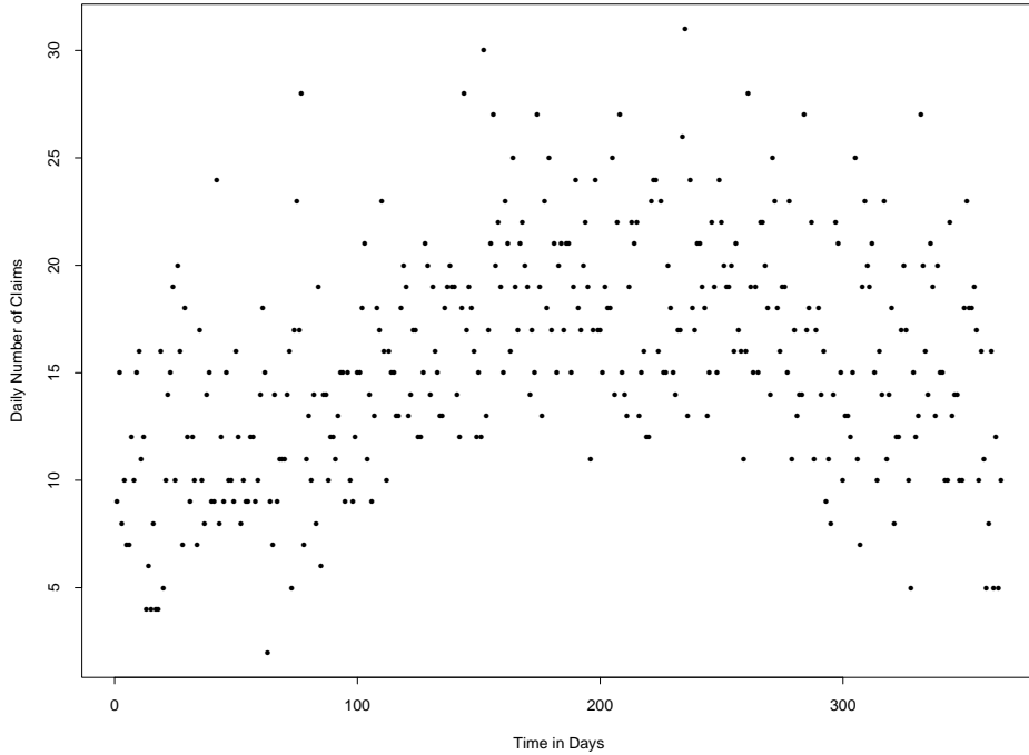
Figure 4: Time series plot of the daily number of claims \Delta_i , i = 1, \dots, 365 , during 1985.
