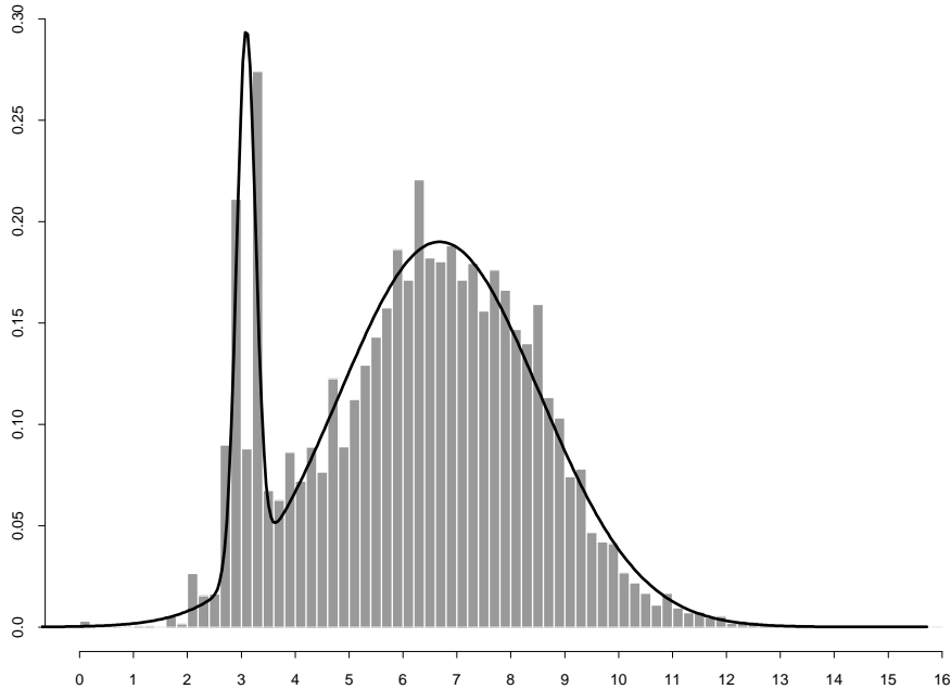
Figure 2: Histogram of all log-instalments and fitted density of bimodal normal mixture model.
