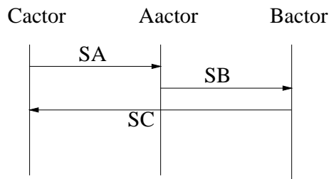
Figure 11: Global Interaction View with event traces
