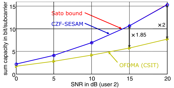
Fig. 7. Sum capacity.
