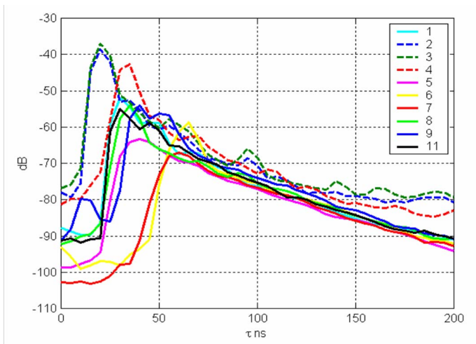
Fig. 6. Power delay profile at different receiver positions normalized to back-to-back level (0 dB).
