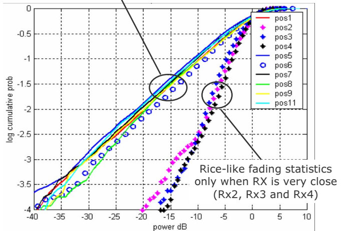
Fig. 4. Fading statistics for different receiver positions.
