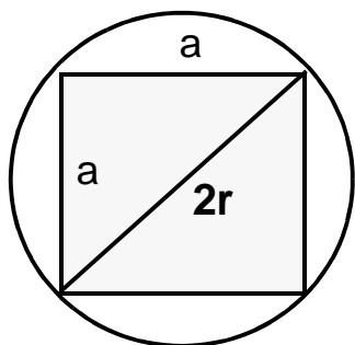
Fig. 3.10 The parameters to calculate the pupil truncation ratio.
