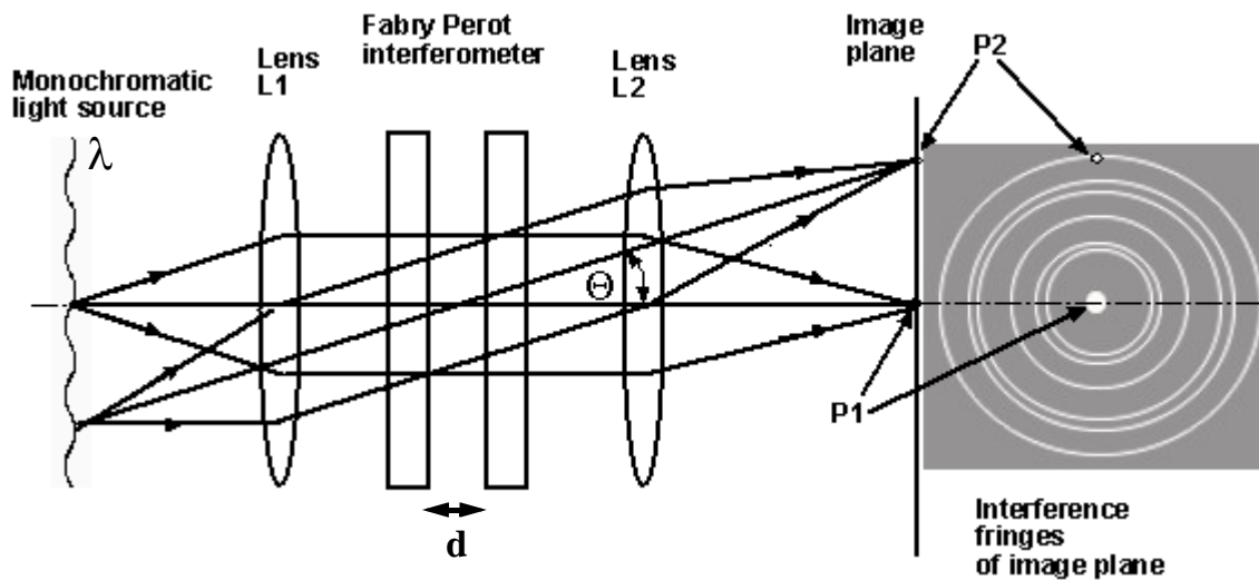
Fig. A.2 An illustration of a basic Fabry-Perot interferometer arrangement. Monochromatic light coming from the left is parallelised by lens L1 , transmitted through the Fabry-Perot and then collimated by lens L2 to image clear and sharp fringes at the detector. The spacing of the plates d and the angle of incident light \Theta are indicated.
