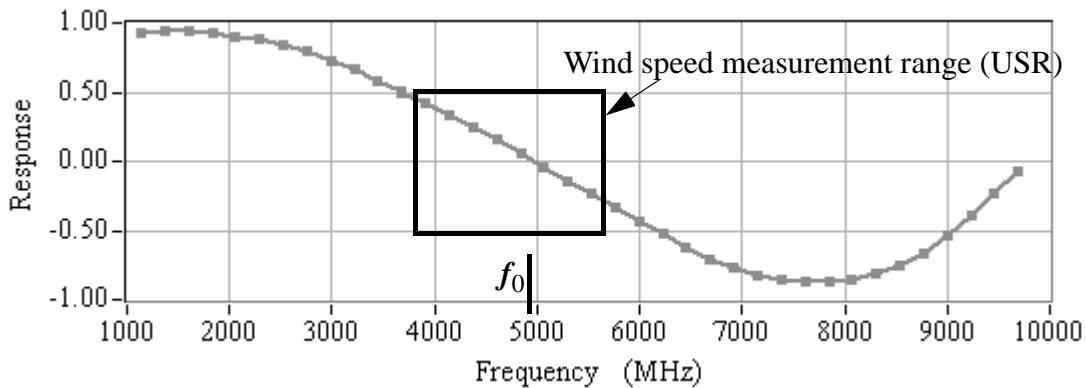
Fig. 5.4 The response values of the transmission transfer functions of Fig. 5.3 versus frequency. The USR of the Mie receiver is the wind measurement range of the instrument.
