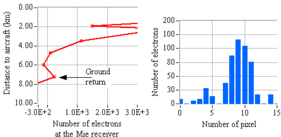
Fig. 5.28 The number of electrons at the Mie receiver for all 16 pixels versus altitude (left) and the number of electrons of the ground return at the Mie receiver versus pixel index (right, Bayerischer Wald, 16:06:22).
