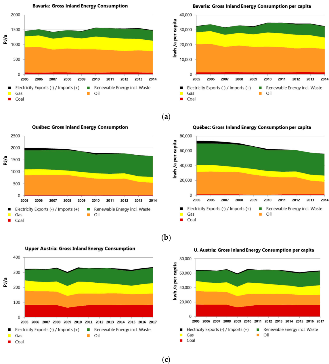
Figure 2. Absolute and per capita gross inland energy consumption in selected RLS partner regions. (a) Bavaria; (b) Québec; (c) Upper Austria. Sources: [40,88,113,114].
