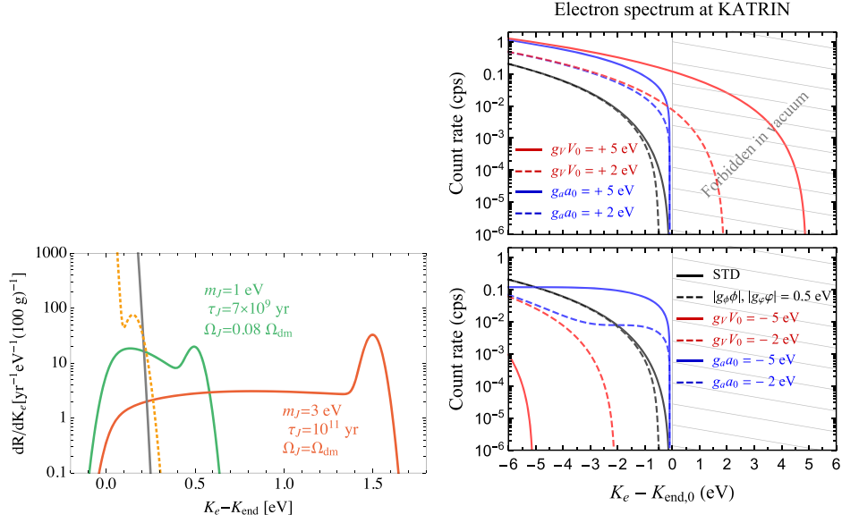
Figure 15. Left: event rates for capture on tritium for neutrinos from Majoron decay J \rightarrow \nu\nu for m_J = 1 \text{ eV} , \tau_J = 7 \times 10^9 \text{ yr} , \Omega_J/\Omega_{\text{dm}} = 0.08 (green, solid) and m_J = 3 \text{ eV} , \tau_J = 10^{11} \text{ yr} , \Omega_J/\Omega_{\text{dm}} = 1 (red, solid) and natural \beta decay (gray, solid) with an electron energy resolution of 0.1 eV. For comparison, we plot the total rate for signal plus background for a Majorana relic-neutrino signal with m_\nu = 0.15 \text{ eV} (yellow, dashed). Reproduced from [115]. CC BY 4.0. Right: the integrated \beta -decay spectra at KATRIN in various types of media: scalar, pseudoscalar and two different vector and axial-vector potentials, with neutrino mass fixed to 0.1 eV. Reproduced from [117]. CC BY 4.0.
