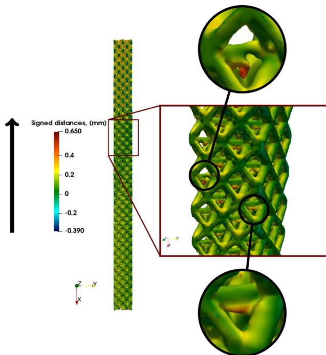
Fig. 10. Comparison of as-manufactured and as-built octet-truss bending specimen 2 \times 32 \times 2 (build direction marked with the black arrow).
