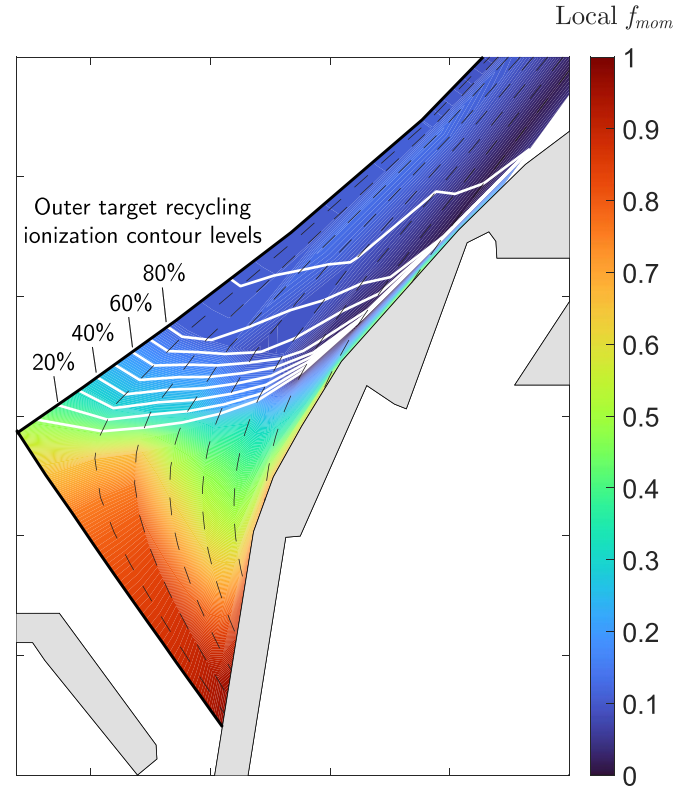
Figure 10. 2D distribution of the local momentum loss factor in the high density, high transport scenario (case B). f_{\text{mom,local}} = 1 means pressure completely removed from a flux tube. White contours represent the fraction of neutrals recycled at the outer target which have ionized after being emitted towards the plasma along any flux tube (each level corresponds to an increase of 10%).
