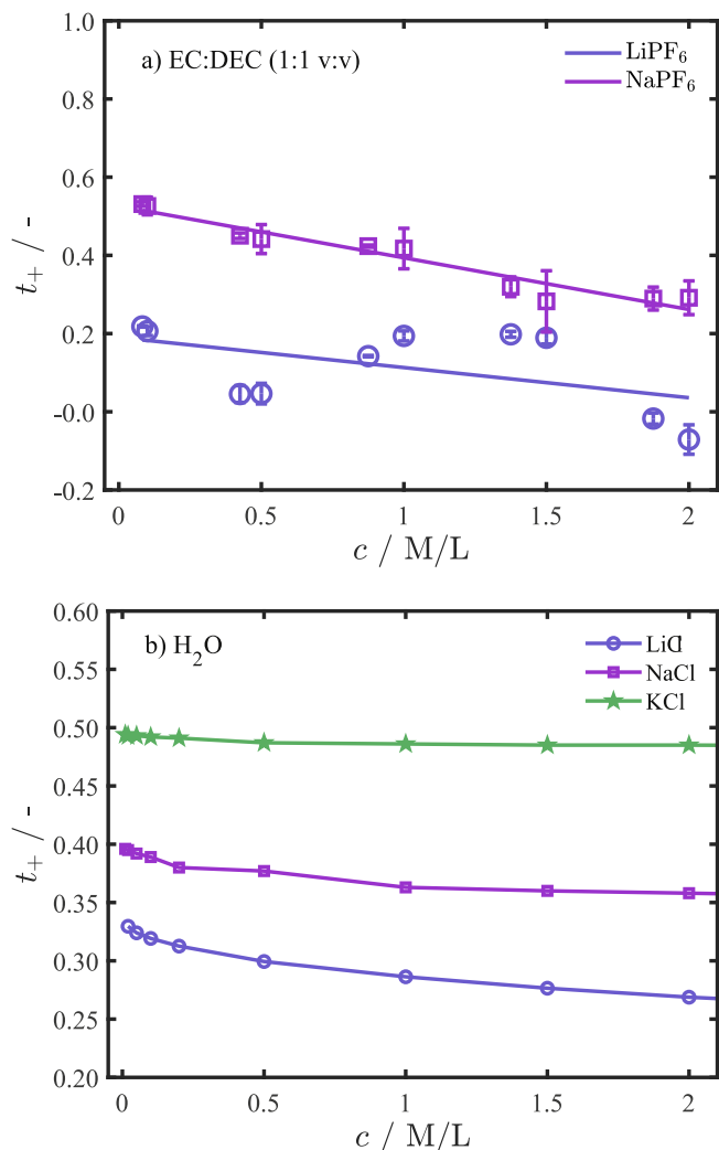
Figure 4. Transference numbers of (a) LiPF 6 and NaPF 6 solutions in EC:DEC (1:1 v:v, 5 wt% FEC was added to sodium electrolytes in coin cells) determined from the transport factors a and b ( t_+(c_0) = 1 - b(c_0)/a(c_0) ), that are shown in the Supporting Information (Figs. S4 and S5) for the EC:DEC (1:1 v:v) based electrolytes with LiPF 6 or NaPF 6 (as detailed in Ref. 21). As shown in Fig. 4a, the cation transference numbers for NaPF 6 in EC:DEC (1:1 v:v) decrease from \approx 0.5 to \approx 0.3 and from \approx 0.2 to \approx 0 for LiPF 6 in EC:DEC (1:1 v:v) decreases from concentrations of 0.1 M to 2.0 M. The here obtained t_+ values for LiPF 6 in EC:DEC (1:1 v:v) are similar to those obtained for EC:EMC (3:7 w:w), where values of t_+ \approx 0.3 at 0.1 M LiPF 6 and t_+ \approx 0.1 at 2.0 M LiPF 6 at 25 °C were obtained. 21 While the trend of decreasing transference number with increasing LiPF 6 concentration is the same, the origin of the absolute difference in transference numbers is currently unknown, and it would require a more detailed investigation to clarify the effect of the various solvents (EC, DMC, DEC, and EMC) and their concentrations on the cation transference number in LiPF 6 based electrolytes. An inspection of the cation transference numbers of LiCl, NaCl, and KCl in H 2 O, shown in Fig. 4b (data from Ref. 31), reveals a similar concentration
