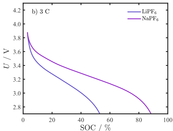
Figure 6. Simulated cell potential vs SOC curves of a hypothetical lithium/sodium “NMC/graphite” cell (using the OCV vs SOC dependence and the kinetic parameters listed in Table S2) during a constant current discharge at different C-rates: (a) at 1 C; (b) at 3 C. Solid lines for LiPF 6 (blue) and NaPF 6 (purple) in EC:DEC (1:1 v:v) are simulated with the measured transport and thermodynamic parameters given in Table I. Additional simulation parameters are given in Table S2. The initial SOC of 3% was chosen to avoid numerical instabilities at the beginning of the discharge simulations.
