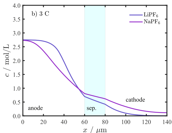
Figure 5. Simulated electrolyte concentration gradients across the cell at the end of discharge (i.e., at a lower cutoff potential of 2.7 V) for a hypothetical lithium/sodium “NMC/graphite” battery (see Table S2): (a) end of 1 C discharge; (b) end of 3 C discharge. The solid lines for LiPF 6 (blue) and NaPF 6 (purple) in EC:DEC (1:1 v:v) are simulated with the measured ionic transport and thermodynamic parameters given in Table I. Additional simulation parameters are given in Table S2. The separator region is highlighted in cyan to easily discern it from the electrodes (see labels in the figure).
