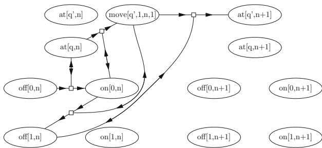
Fig. 1 Some of the states and transitions involved in modelling a Turing machine
