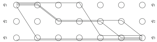
Fig. 2 Realizable history in IO protocol with three states
