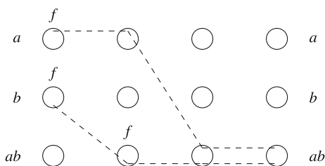
Fig. 7 History H of Fig. 4 after pruning
