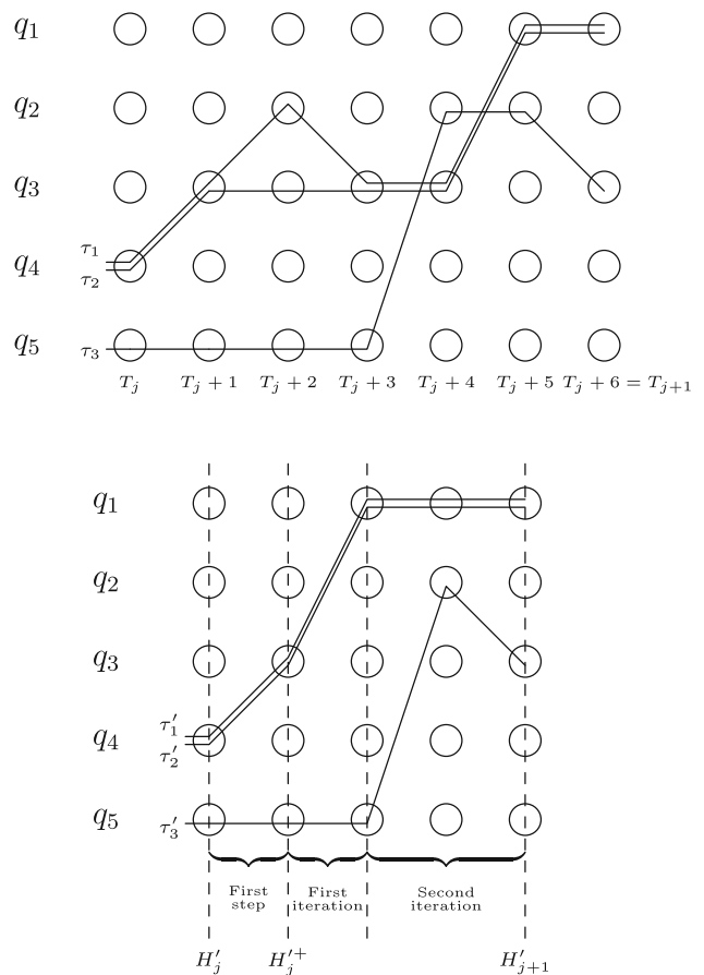
Fig. 5 Illustration of the proof of Theorem 4.33
