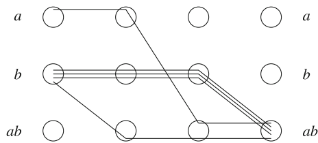
Fig. 4 Realizable history in \mathcal{P}_{MFDO} of Example 4.3
