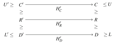
Fig. 6 Construction of the proof of Lemma 5.3
