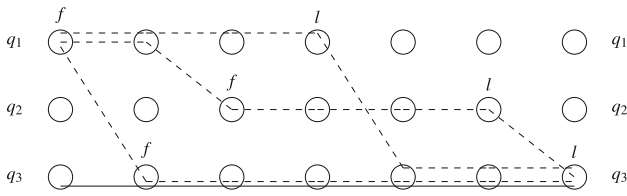
Fig. 3 History H of Fig. 2 after pruning
