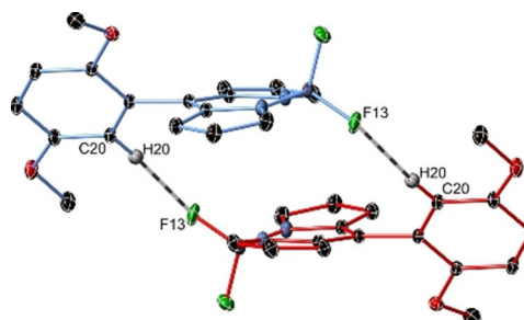
Figure 4. The dimeric C–H \cdots F of 3.292 Å (C20–F13) interaction observed within the crystal structure of BDP-5 ; the symmetry-equivalent red and blue molecules are related by an inversion center. Thermal ellipsoids are shown at the 50% probability level, H-atoms not involved in this interaction have been omitted.
