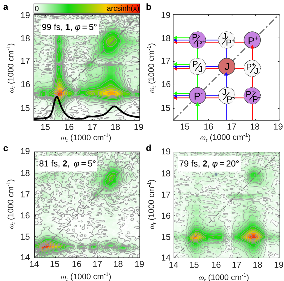
Fig. 3 Sample- and angle-dependence of the observed dynamics. a The 2D spectrum of sample 1 at T=100 fs and \varphi = 5^\circ . b A schematic 2D plot visualises the labelling of the on-diagonal- and cross-peaks, and highlights the distinction between signals: polaritonic states (purple), excitonic state (red), excitonic-polaritonic cross-peaks (white). The arrows indicate how to read out the 2D spectrum with excitation on the x-axis and detection on the y-axis. c The 2D spectra of sample 2 at T=80 fs and \varphi = 5^\circ and d at \varphi = 20^\circ show that the transient behaviour depends on the cavity tuning (by comparison to sample 1 in a ), as well as where along k_{\parallel} the excitation/detection takes place. The data in a , c , and d is scaled by an arcsinh-function to visualise a larger dynamic range.
